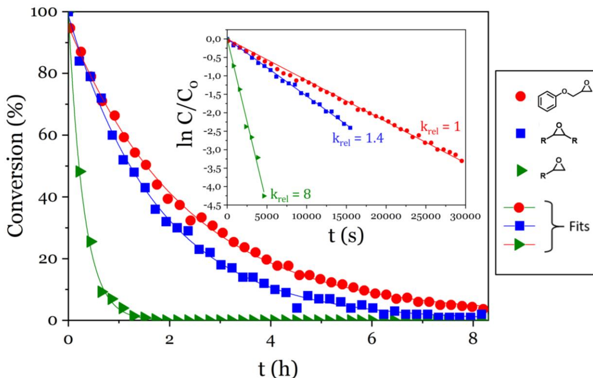
Figure 1. Evolution of the conversion of the epoxy model molecules versus time and pseudo-first order plots (inset).
