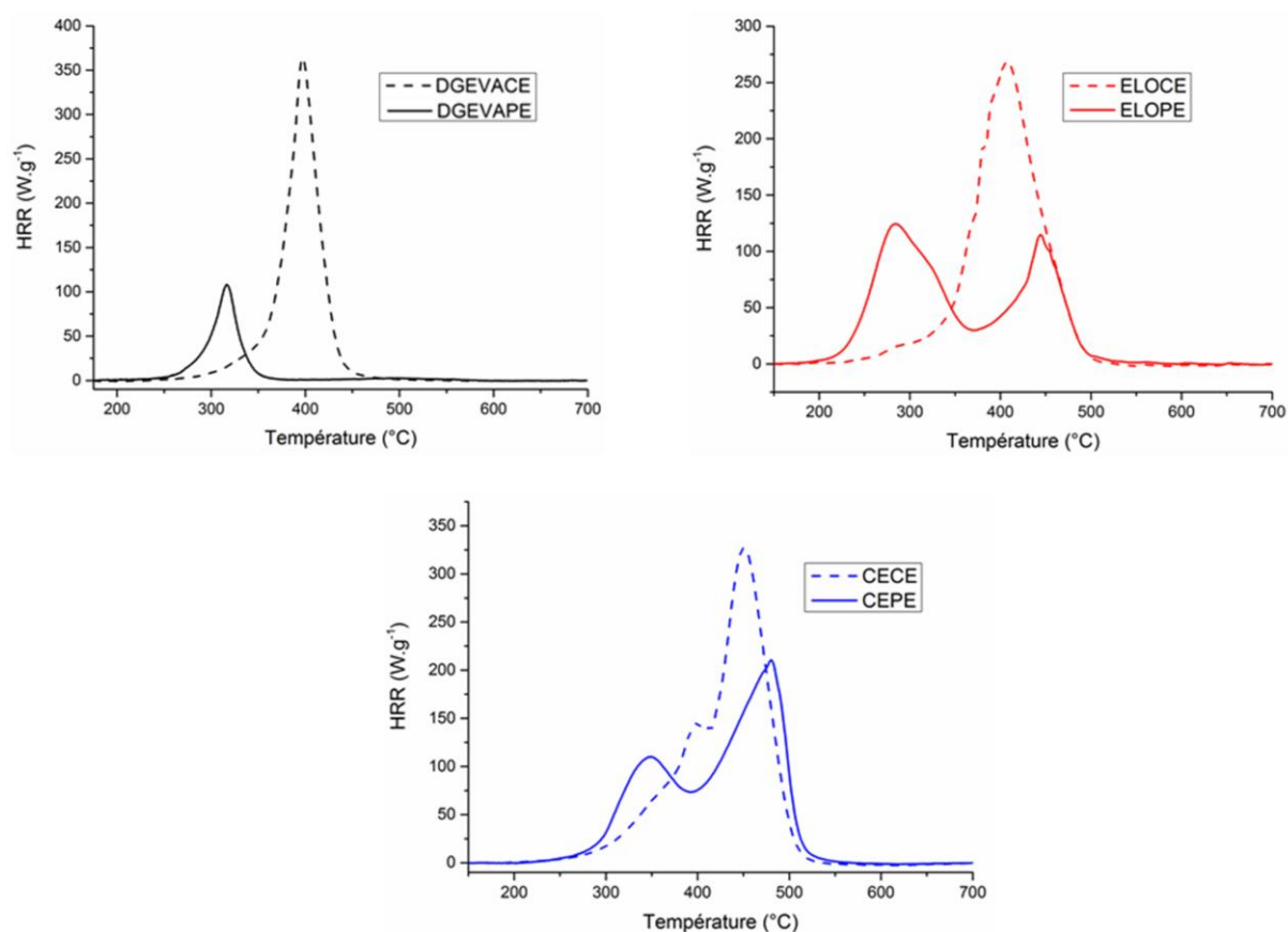
Figure 6: PCFC curves of the phosphate ester vitrimers DGEVAPE, ELOPE, CEPE and their carboxylic ester counterparts DGEVACE, ELOCE and CECE.
