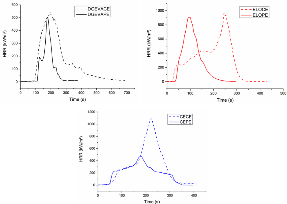
Figure 8: Cone calorimeter curves of the phosphate ester vitrimers DGEVAPE, ELOPE, CEPE and their carboxylic ester counterparts DGEVACE, ELOCE, CECE.
