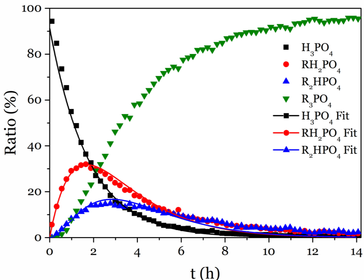
Figure 2. Evolution with time of the proportion of P-containing species during the reaction of phosphoric acid with phenyl glycidyl epoxy.
