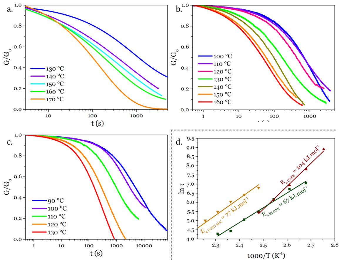
Figure 5. Stress-relaxation experiments results on a. DGEVAPE, b. ELOPE and c. CEPE. d. Arrhenius diagram of the \tau determined from Kohlrausch-Williams-Watt fits for each material, and determination of the flow activation energies.
