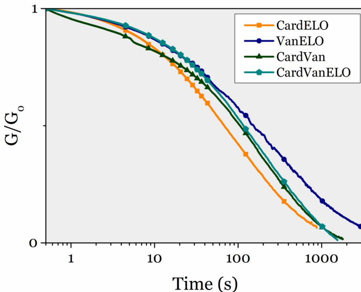
Figure 10. Stress-relaxation experiments on epoxy mixtures vitrimers at 150 °C.
