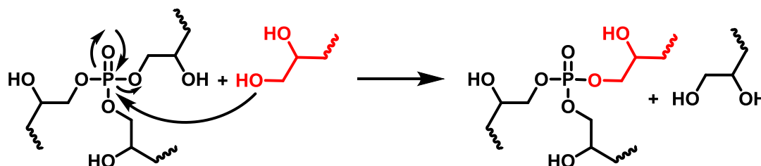
Figure 4. Exchange in the polymer network by phosphate transesterification.
