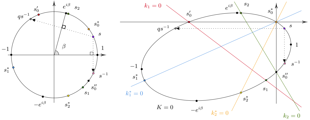
Figure 3: On the left, the points introduced in Lemmas 3 and 14 on the unit complex circle \mathbb{U} ; on the right, their images by (\mathbf{x}, \mathbf{y}) on the ellipse S \cap \mathbb{R}^2 . For the sake of readability, points on the ellipse are labelled with their preimages. Invariances in (22) are represented by the dotted arrows.
