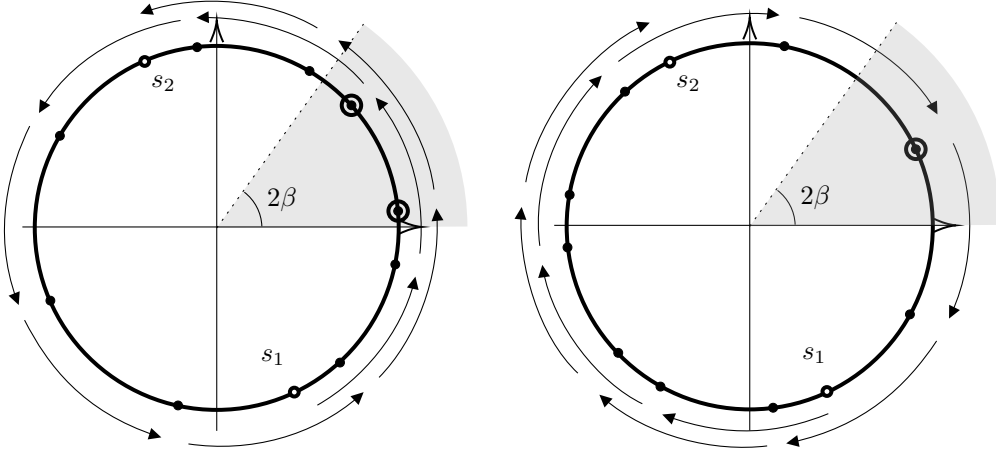
Figure 5: Enumeration of \mathbf{P} and \mathbf{Z} for (d, r) = (-9, 2) (on the left) and (d, r) = (11, -1) (on the right). The shaded area corresponds to \mathbf{y}^{-1}(\overline{\mathcal{G}}_{\mathcal{H}}) .
