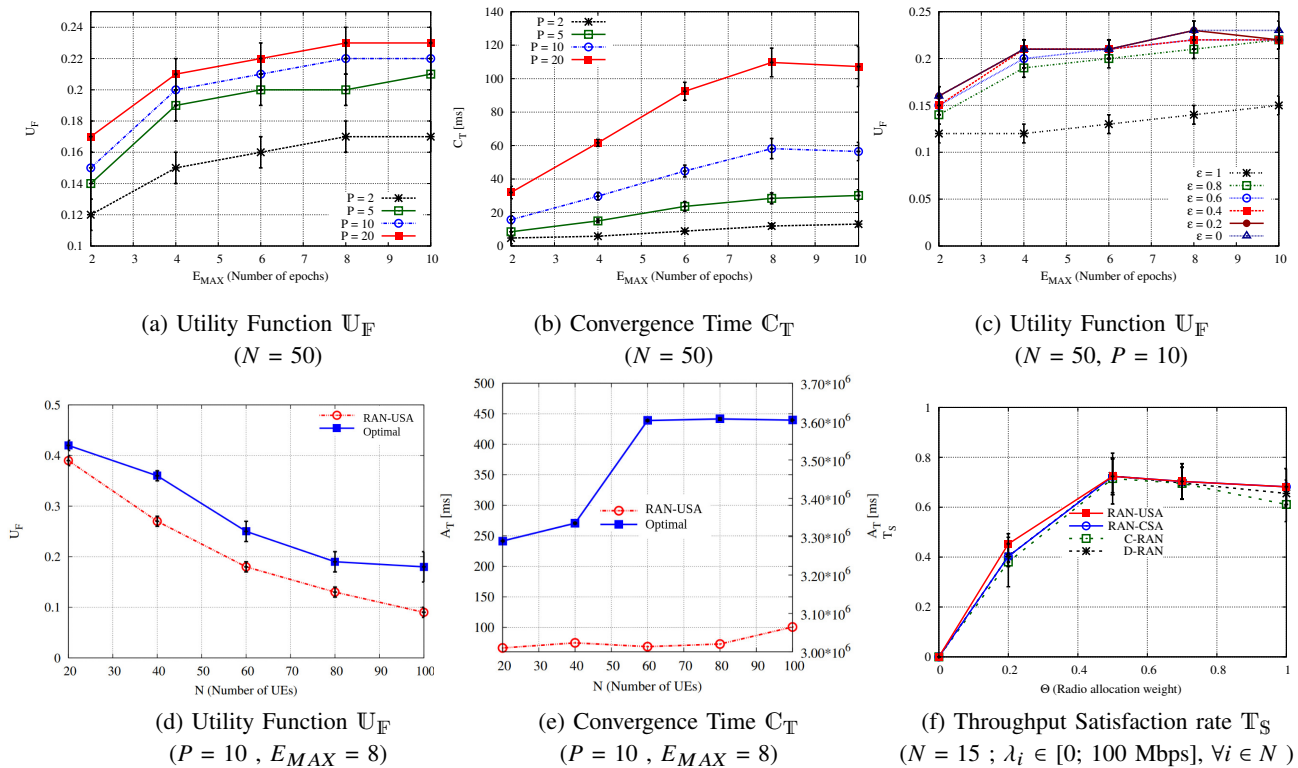
Fig. 4: Convergence evaluation
