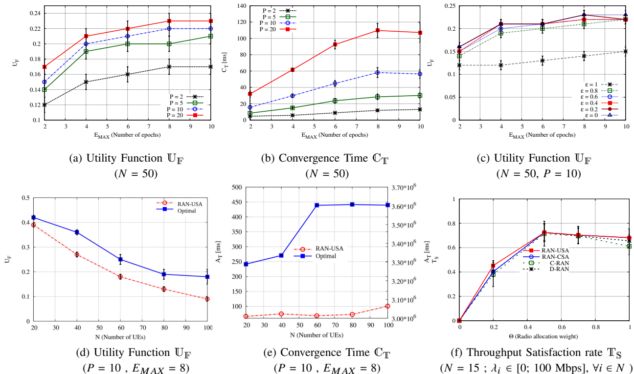
Fig. 4: Convergence evaluation
