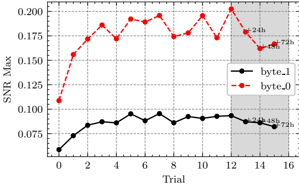
Fig. 9: Evolution of the SNR of Byte 0 and Byte 1 after irradiation of Byte 1 every 10 minutes of irradiation
