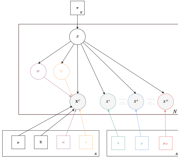
Figure 1: Graphical representation of our Model (18), with colors for additions/variants from Gaussian distribution. One color per continuous law for additional latent variables and parameters, and one color per type of discrete law: Student distribution (orange), SAL distribution (purple), Poisson (green), Bernoulli (blue) and Multinomial (red).
