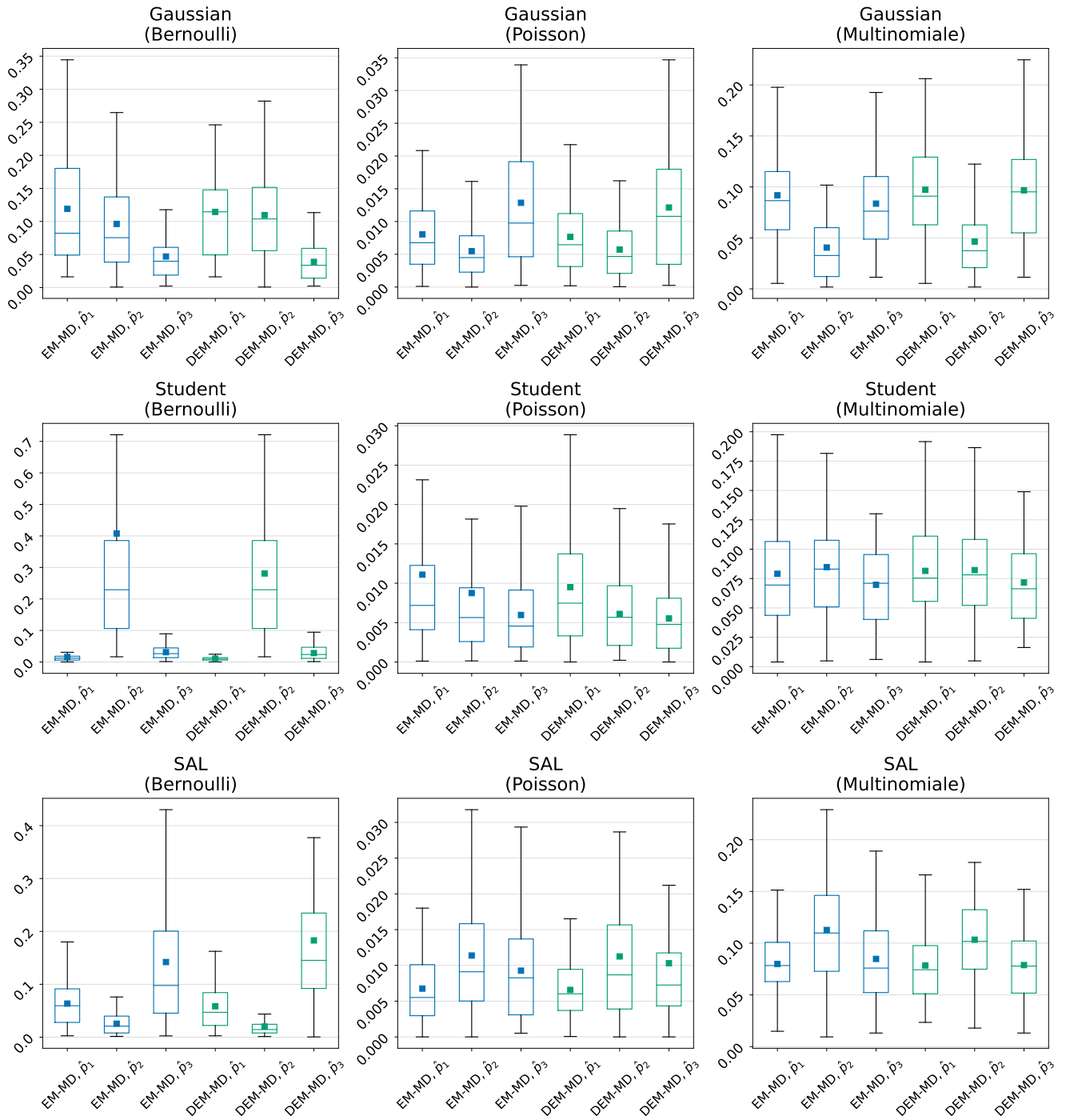
Figure 4: Boxplots of relative discrete distribution parameter errors for settings C_{223} (a) and C_{343} (b), for the three DEM-MD on both DEM-MD (green) and EM-MD (blue). In each subplot, a row corresponds to a continuous distribution (Gaussian, Student, SAL in this order).
