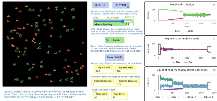
Fig. 1. Habits simulator interface: world (left), actions (middle) and plots (right)
