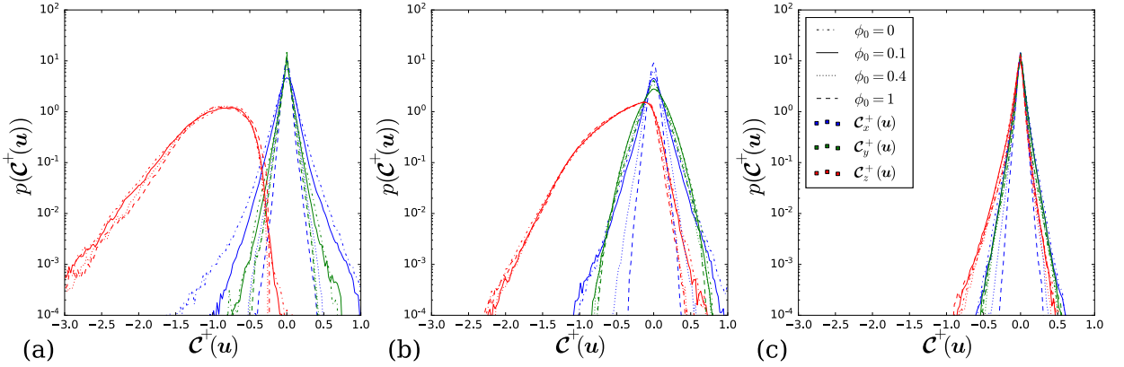
Figure 3: PDF of fluid vorticity, normalised by the viscous time scale, for different mass loadings with St^+ = 7 , in the (a) viscous sublayer, (b) buffer layer and (c) log layer. The line colour indicates the component of the vorticity, and the line style indicates the mass loading.
