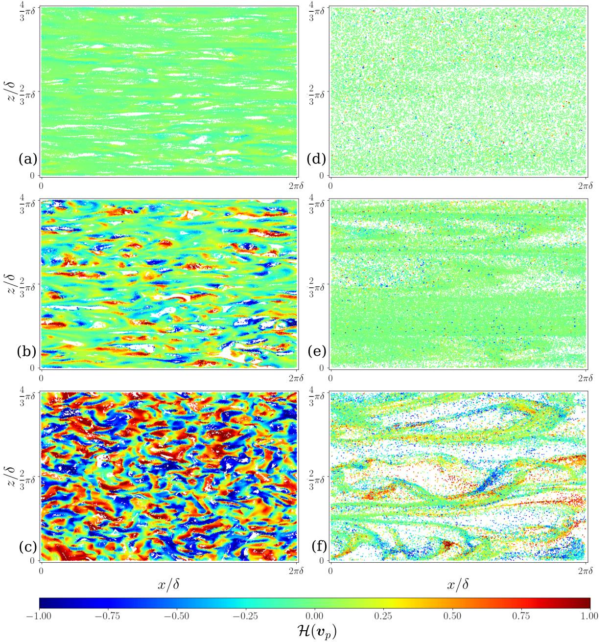
Figure 9: Particle positions coloured by relative helicity in wall-parallel slices, for (a) viscous sublayer, St^+ = 3 , \phi_0 = 1 ; (b) buffer layer, St^+ = 3 , \phi_0 = 1 ; (c) log layer, St^+ = 3 , \phi_0 = 1 ; (d) viscous sublayer, St^+ = 60 , \phi_0 = 1 ; (e) buffer layer, St^+ = 60 , \phi_0 = 1 ; (f) log layer, St^+ = 60 , \phi_0 = 1 . Thickness of the layers used are defined in figure 7.
