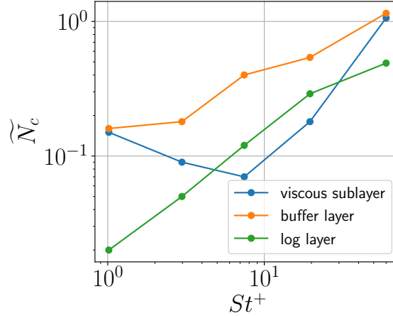
Figure 12: Collision rate non-dimensionalized according to equation 15 for various Stokes numbers with \phi_0 = 1 .
