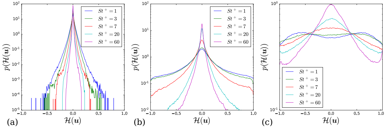
Figure 6: PDF of fluid relative helicity for various Stokes numbers with \phi_0 = 1 , in the (a) viscous sublayer, (b) buffer layer and (c) log layer. Note that the y -axis ranges for each PDF are different.
