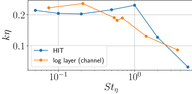
Figure 22: Wavenumber of maximum in spectra of particle number density fluctuations as a function of Kolmogorov Stokes number for HIT (Matsuda et al. , 2014) and the logarithmic layer in the present dataset.
