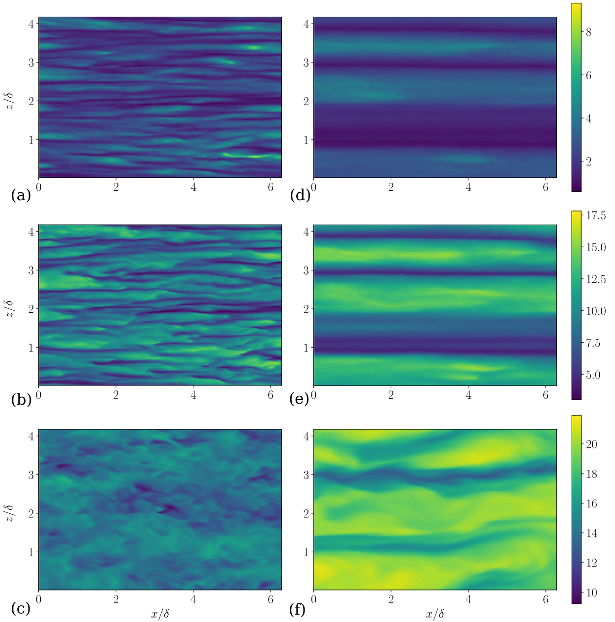
Figure 26: Fluid streamwise velocity u^+ for (a) \phi_0 = 1.0 , St^+ = 3 at y^+ = 2.5 ; (b) \phi_0 = 1.0 , St^+ = 3 at y^+ = 12 ; (c) \phi_0 = 1.0 , St^+ = 3 at y^+ = 100 ; (d) \phi_0 = 1.0 , St^+ = 60 at y^+ = 2.5 ; (e) \phi_0 = 1.0 , St^+ = 60 at y^+ = 12 ; (f) \phi_0 = 1.0 , St^+ = 60 at y^+ = 100 .
