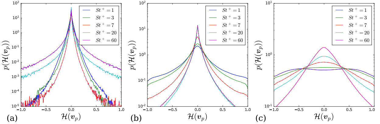
Figure 14: PDFs of the relative helicity (cosine of the angle between particle velocity and vorticity) \mathcal{H}(\mathbf{v}_p) of the particles for various Stokes numbers with \phi_0 = 1 , in the (a) viscous sublayer, (b) buffer layer, and (c) log layer. Note that the y-ranges differ by orders of magnitude.
