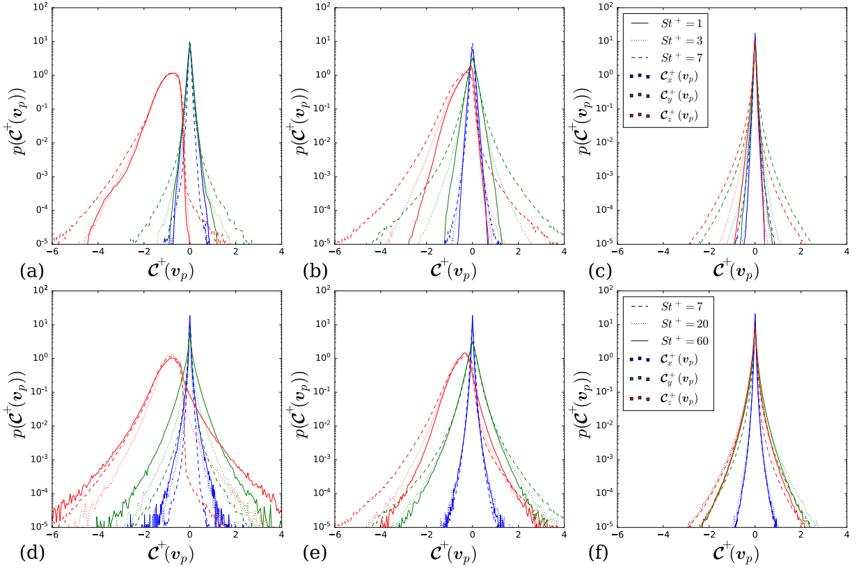
Figure 13: PDF of particle velocity curl, normalised by the viscous time scale, for a range of Stokes numbers with \phi_0 = 1 . Data for small Stokes numbers: (a) viscous sublayer, (b) buffer layer and (c) log layer. Data for large Stokes numbers: (d) viscous sublayer, (e) buffer layer and (f) log layer. The line colour indicates the component of the curl, and the line style indicates the Stokes number.
