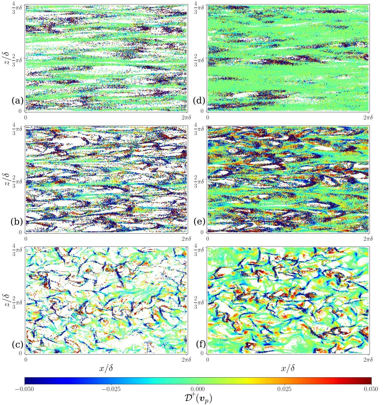
Figure 15: Particle positions coloured by divergence in wall-parallel slices, for (a) viscous sublayer, \phi_0 = 0.1 , St^+ = 7 ; (b) buffer layer, \phi_0 = 0.1 , St^+ = 7 ; (c) log layer, \phi_0 = 0.1 , St^+ = 7 ; (d) viscous sublayer, \phi_0 = 0.4 , St^+ = 7 ; (e) buffer layer, \phi_0 = 0.4 , St^+ = 7 ; (f) log layer, \phi_0 = 0.4 , St^+ = 7 . Divergence is normalised by the viscous time scale, and the colour bar is truncated to emphasise regions of zero divergence. The slices used for visualisation are 2 \leq y^+ < 3 , 9.5 \leq y^+ < 14.5 and 97.5 \leq y^+ < 102.5 for viscous sublayer, buffer layer, and log layer, respectively.
