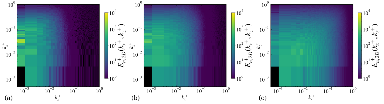
Figure 24: 2D Fourier spectra of particle number density on 2D slices in (a) viscous sublayer, (b) buffer, and (c) log layers for \phi_0 = 1.0 and St^+ = 7 . The spectra and the wavenumber are normalised by the viscous length scale. Areas appearing in black indicate regions where there is no particle distribution.
