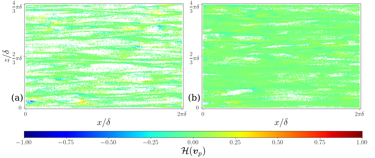
Figure 20: Particle positions coloured by relative helicity in wall-parallel slices, for (a) viscous sublayer, \phi_0 = 0.1 , St^+ = 7 ; (b) viscous sublayer, \phi_0 = 0.4 , St^+ = 7 .
