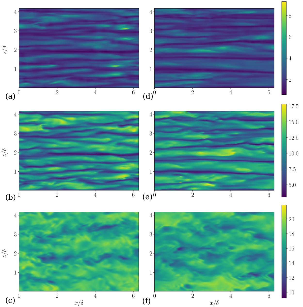
Figure 25: Fluid streamwise velocity u^+ for (a) \phi_0 = 0.1 , St^+ = 7 at y^+ = 2.5 ; (b) \phi_0 = 0.1 , St^+ = 7 at y^+ = 12 ; (c) \phi_0 = 0.1 , St^+ = 7 at y^+ = 100 ; (d) \phi_0 = 0.4 , St^+ = 7 at y^+ = 2.5 ; (e) \phi_0 = 0.4 , St^+ = 7 at y^+ = 12 ; (f) \phi_0 = 0.4 , St^+ = 7 at y^+ = 100 .
