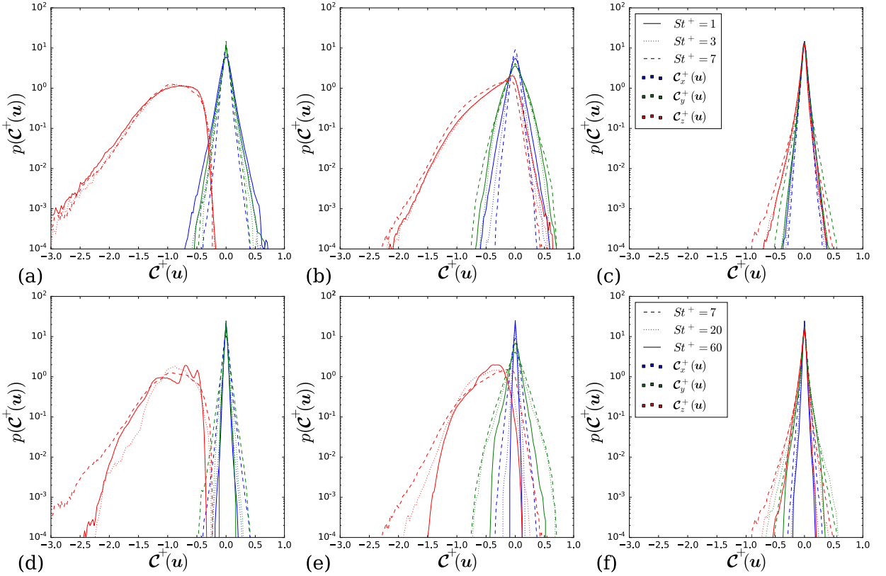
Figure 4: PDF of fluid vorticity, normalised by the viscous time scale, for a range of Stokes numbers with \phi_0 = 1 . Data for small Stokes numbers: (a) viscous sublayer, (b) buffer layer and (c) log layer. Data for large Stokes numbers: (d) viscous sublayer, (e) buffer layer and (f) log layer. The line colour indicates the component of the vorticity, and the line style indicates the Stokes number.
