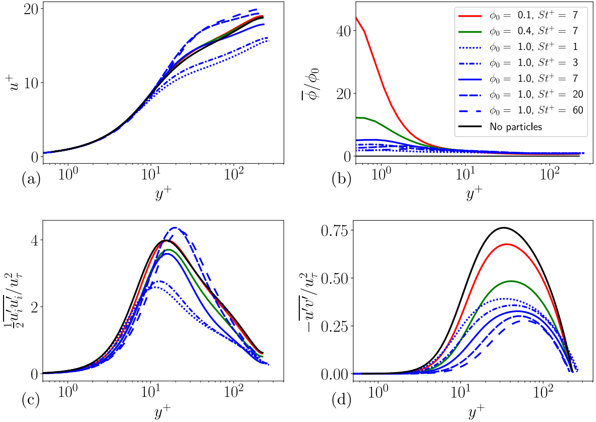
Figure 2: (a) Mean streamwise fluid velocity, u^+ , as a function of wall-normal distance, y^+ , for various mass loadings and Stokes numbers, as well as without particles. (b) Local mean mass loading. (c) Fluid phase turbulent kinetic energy (TKE). (d) Fluid phase Reynolds shear stress ( u'v' ). The legend in (b) applies to all sub-figures.
