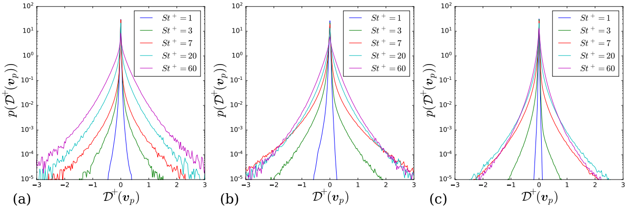
Figure 11: PDF of particle velocity divergence, normalised by the viscous time scale, for various Stokes numbers with \phi_0 = 1 , in the (a) viscous sublayer, (b) buffer layer, and (c) log layer.
