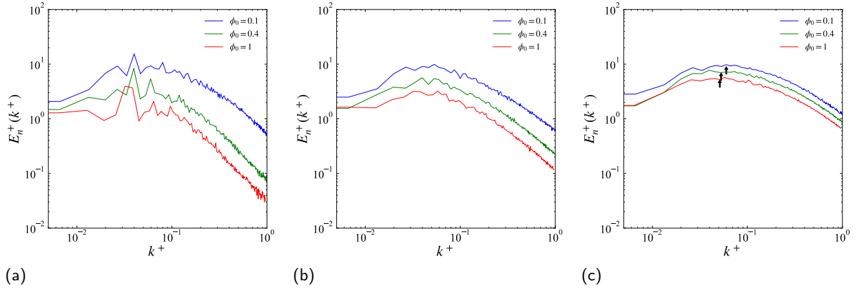
Figure 23: Fourier spectra of particle number density on 2D slices in (a) viscous sublayer, (b) buffer, and (c) log layers for various mass loadings with St^+ = 7 . The spectra and the wavenumber are normalised by the viscous length scale. In (c), the peak locations obtained with a five-point moving average are indicated with arrows.
