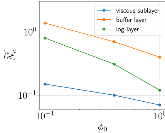
Figure 17: Collision rate non-dimensionalized according to equation 15 for various mass loadings with St^+ = 7 .
