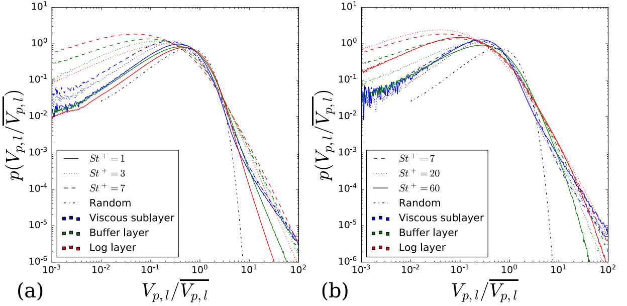
Figure 10: PDF of modified Voronoi volume as a function of flow region and Stokes number, normalised by the mean modified Voronoi volume within each layer for (a) St^+ = 1, 3, 7 ; \phi_0 = 1 , and (b) St^+ = 7, 20, 60 ; \phi_0 = 1 . The dashed-dotted line represents the volume distribution for randomly distributed particles.
