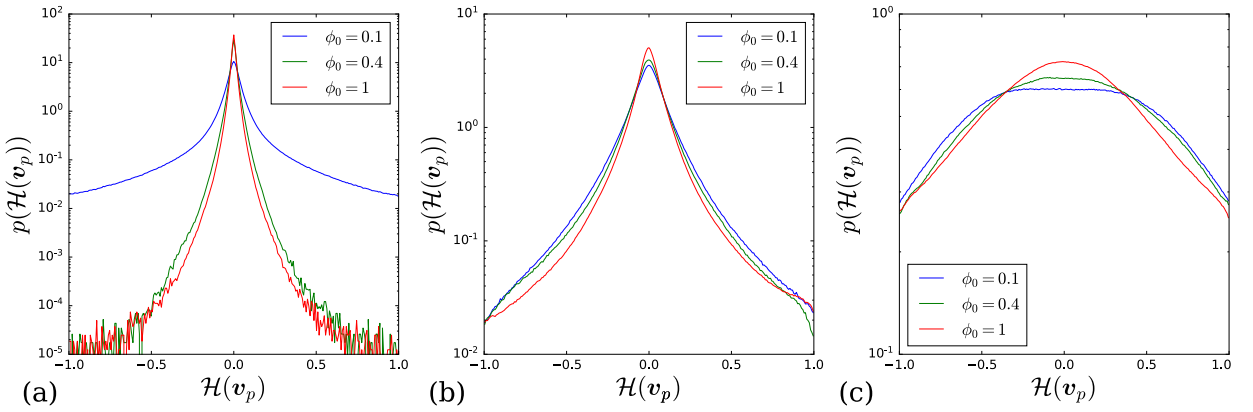
Figure 19: PDFs of the relative helicity \mathcal{H}(v_p) of the particles for different mass loadings with St^+ = 7 , in the (a) viscous sublayer, (b) buffer layer and (c) log layer. Note that the y -ranges differ by orders of magnitude.
