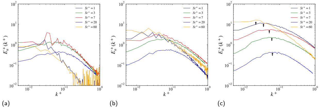
Figure 21: Fourier spectra of particle number density in 2D slices in (a) viscous sublayer, (b) buffer, and (c) log layers for various Stokes numbers with \phi_0 = 1 . The spectra and the wavenumber are normalised by the viscous length scale. In (c), the peak locations obtained with a five-point moving average are indicated with arrows.
