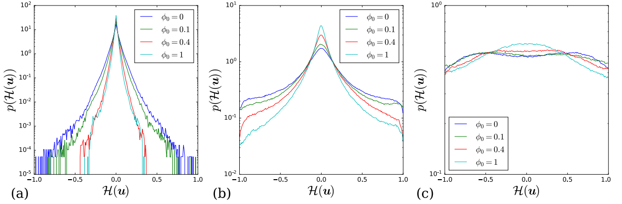
Figure 5: PDF of fluid relative helicity for various mass loadings with St^+ = , in the (a) viscous sublayer, (b) buffer layer and (c) log layer. Note that the y -axis ranges for each PDF are different.
