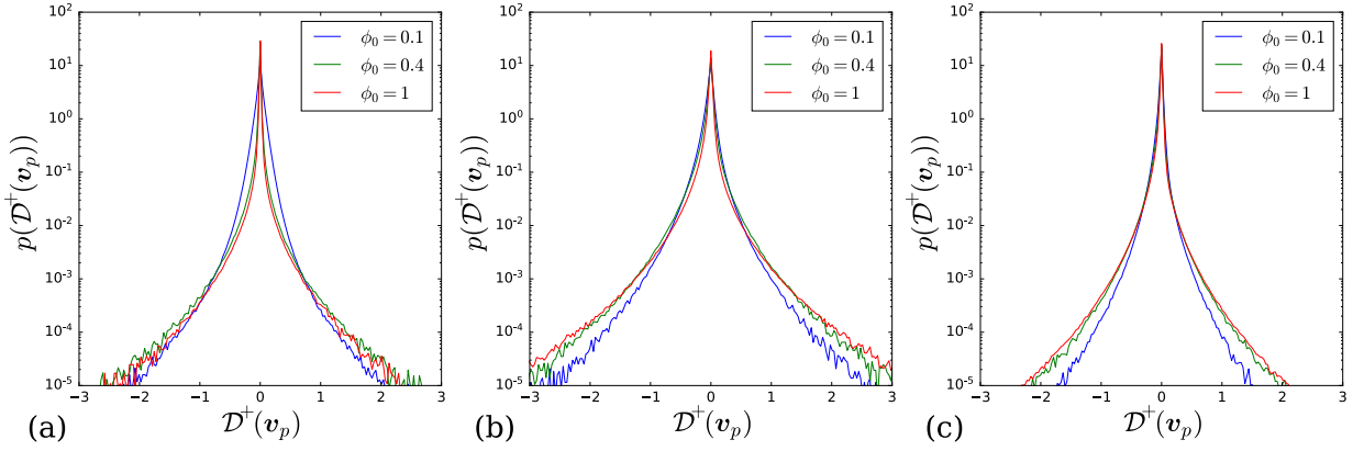
Figure 16: PDF of particle velocity divergence, normalised by the viscous time scale, for three different mass loadings with St^+ = 7 , in the (a) viscous sublayer, (b) buffer layer, and (c) log layer.
