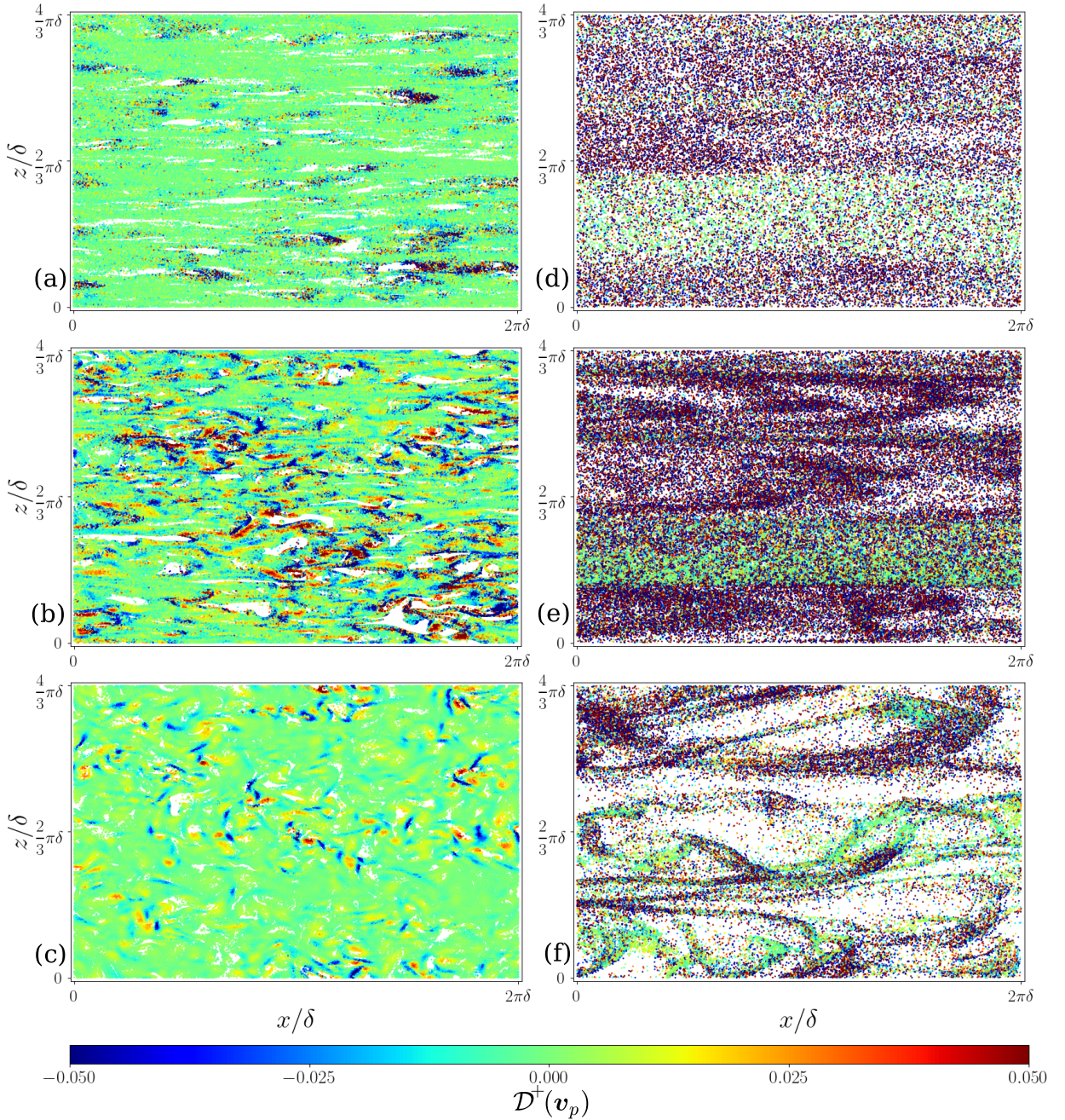
Figure 7: Particle positions coloured by divergence in wall-parallel slices, for (a) viscous sublayer, Sr^+ = 3 , \phi_0 = 1 ; (b) buffer layer, Sr^+ = 3 , \phi_0 = 1 ; (c) log layer, Sr^+ = 3 , \phi_0 = 1 ; (d) viscous sublayer, Sr^+ = 60 , \phi_0 = 1 ; (e) buffer layer, Sr^+ = 60 , \phi_0 = 1 ; (f) log layer, Sr^+ = 60 , \phi_0 = 1 . Divergence is normalised by the viscous time scale, and the colour bar is truncated to emphasise regions of zero divergence. Because of the difference in number density, thinner slices are used to visualise the Sr^+ = 3 data. The slices used for Sr^+ = 3 are 2.375 \leq y^+ < 2.625 , 11.375 \leq y^+ < 12.625 and 99.375 \leq y^+ < 100.625 for viscous sublayer, buffer layer and log layer, respectively. The slices used for Sr^+ = 60 are 2 \leq y^+ < 3 , 9.5 \leq y^+ < 14.5 and 97.5 \leq y^+ < 102.5 for viscous sublayer, buffer layer and log layer, respectively.
