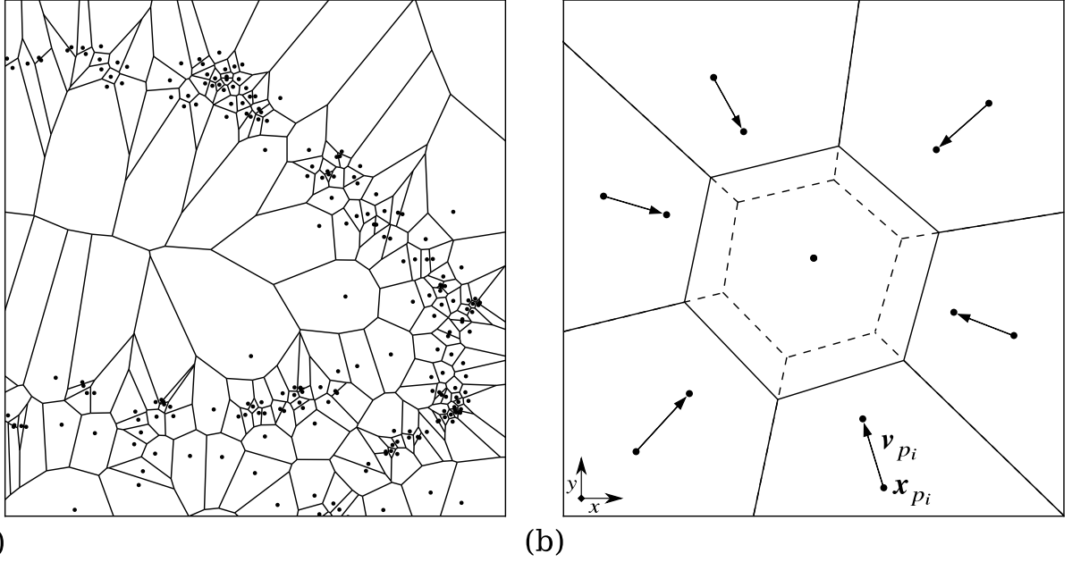
Figure 1: (a) Voronoi tessellation in 2D for a cluster of particles. (b) Example of the motion of a two-dimensional modified Voronoi tessellation at two subsequent time instants for a converging cluster. The solid line corresponds to the time step t^k and the dashed line to t^{k+1} .
