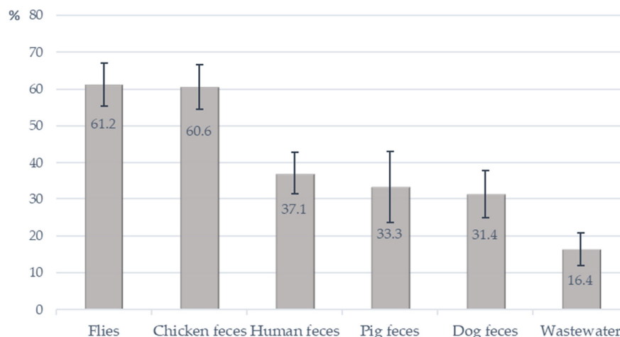
Figure 2. Detection of OptrA -positive E. faecalis from investigated farms.
