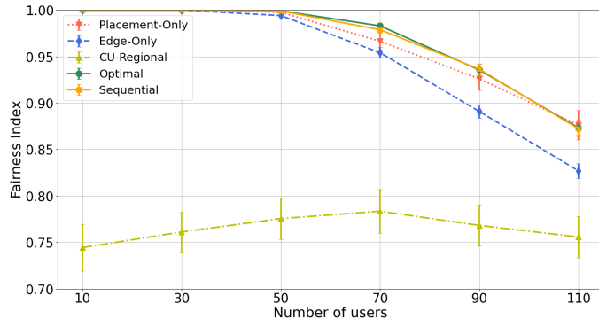
Figure 5: User fairness as a function of the number of users.
