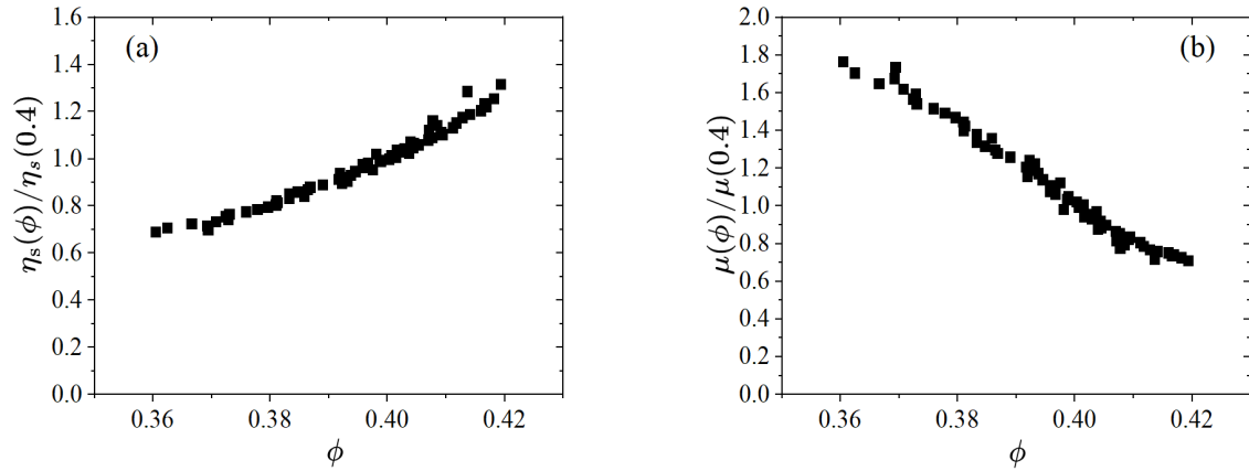
FIG. 10. Local variation of the viscosity (a) and of the apparent friction coefficient (b) as a function of the local volume fraction for a 40% suspension.
