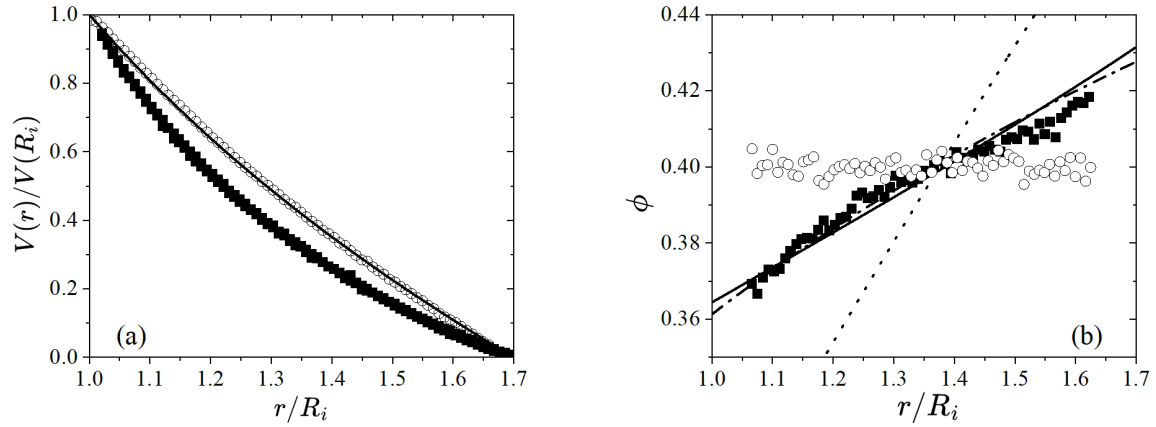
FIG. 9. Initial (empty circles) and steady (squares) velocity (a) and concentration (b) profiles for a 40% suspension. The full line in (a) is the theoretical velocity profile for a homogeneous Newtonian fluid. The lines in (b) are the predictions of the SBM with the three sets of equations described in Sec. IV [(i): dashed-dotted line, (ii): solid line, and (iii): dotted line].
