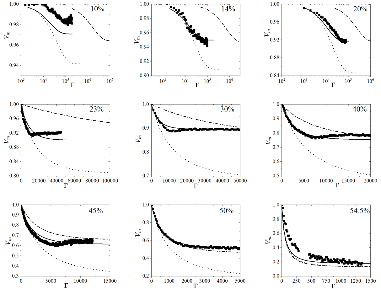
FIG. 7. Evolution of the velocity V_m in the middle of the gap as a function of the macroscopic strain \Gamma = \Omega t : experimental data (squares) and predictions of the SBM (lines) with the three sets of equations described in the text [(i): dashed-dotted line, (ii): solid line, and (iii): dotted line]. The average volume fraction of the studied suspension is, from left to right and from top to bottom: 10%, 14%, 20%, 23%, 30%, 40%, 45%, 50%, 54.5%. A semi-log scale is used for clarity for \phi \lesssim 20\% .
