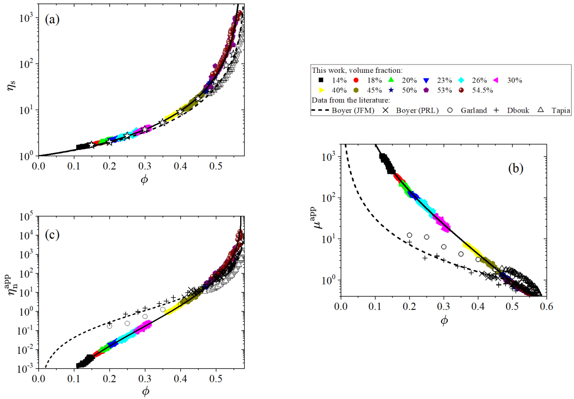
FIG. 2. (a) Local dimensionless viscosity \eta_s , (b) apparent friction coefficient \mu^{\text{app}} , and (c) apparent normal viscosity \eta_n^{\text{app}} as a function of the local volume fraction \phi , from experiments performed at various average volume fraction (see legend). Macroscopic measurements from the literature by Dbouk, Lobry, and Lemaire 30 , Garland et al. 31 , Boyer, Guazzelli, and Pouliquen 32 , Tapia, Pouliquen, and Guazzelli 34 , Boyer, Pouliquen, and Guazzelli 38 are also shown (see legend). For clarity, only the data of Boyer, Pouliquen, and Guazzelli 38 and Tapia, Pouliquen, and Guazzelli 34 are shown in (a). We recall that \eta_n^{\text{app}} and \mu^{\text{app}} are deduced from the steady-state volume fraction profiles under the assumption that there is no additional diffusion term in the SBM. The dashed lines are the rheological laws – Eqs. (B1), (B2) and (B3) – of Boyer, Guazzelli, and Pouliquen 32 . The full lines are the phenomenological laws Eqs. (13), (14) and (15).
