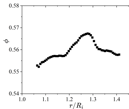
FIG. 14. Initial volume fraction profile (after loading) of a 56% suspension in a wide gap Couette geometry of inner radius 4.1 cm and outer radius 6 cm, slightly different from that used in the rest of the paper.
