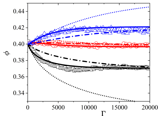
FIG. 13. Evolution of the local volume fraction as a function of the macroscopic strain \Gamma = \Omega t for a 40% suspension, at various dimensionless radial positions r/R_i in the gap of the Couette geometry: experimental data (symbols) and predictions of the SBM (lines) with the three sets of equations described in Sec. IV [(i): dashed-dotted line, (ii): solid line, and (iii): dotted line]. Data are taken at r/R_i = 1.07 (black lines and squares), r/R_i = 1.35 (red lines and circles) and r/R_i = 1.6 (blue lines and triangles); we recall that the outer wall location is R_o/R_i = 1.7 . The local concentrations are computed here from the velocity profiles, as described in the text.
