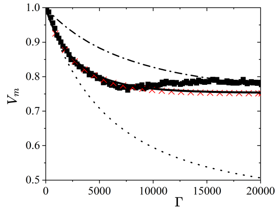
FIG. 12. Evolution of the velocity V_m in the middle of the gap as a function of the macroscopic strain \Gamma = \Omega t for a 40% suspension: experimental data (squares) and predictions of the SBM (lines) with the three sets of equations described in Sec. IV [(i): dashed-dotted line, (ii): solid line, and (iii): dotted line]. The red crosses show the best fit of the data to the SBM in its simplest form ( D_{12} = 0 in Eq. (A10)), which leads to the apparent friction coefficient data shown in Fig. 5 in the range [37%,42%].
