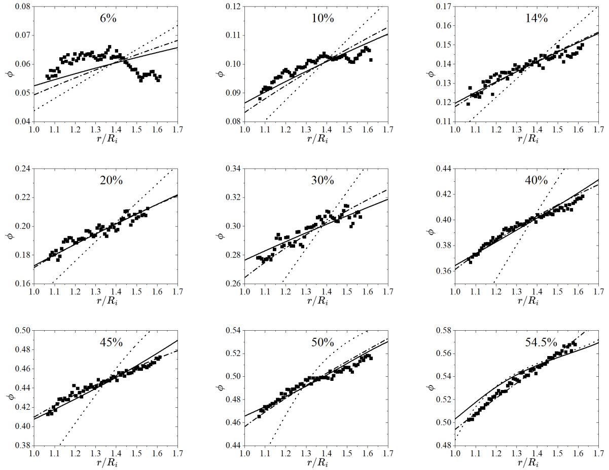
FIG. 6. Steady state volume fraction profiles: experimental data (squares) and predictions of the SBM (lines) with the three sets of equations described in the text [(i): dashed-dotted line, (ii): solid line, and (iii): dotted line]. The average volume fraction of the studied suspension is, from left to right and from top to bottom: 6%, 10%, 14%, 20%, 30%, 40%, 45%, 50%, 54.5%.
