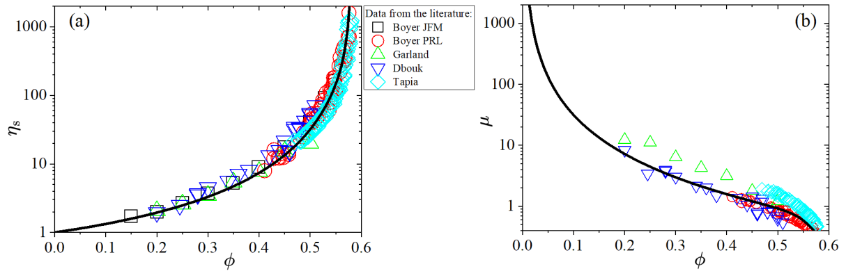
FIG. 8. Macroscopic measurements from the literature by Dbouk, Lobry, and Lemaire 30 , Garland et al. 31 , Boyer, Guazzelli, and Pouliquen 32 , Tapia, Pouliquen, and Guazzelli 34 , Boyer, Pouliquen, and Guazzelli 38 (see legend). (a) Dimensionless viscosity \eta_s , and (b) friction coefficient \mu as a function of volume fraction \phi . The lines are the rheological laws – Eqs. (B1), (B2) and (B3) – of Boyer, Guazzelli, and Pouliquen 32 .
