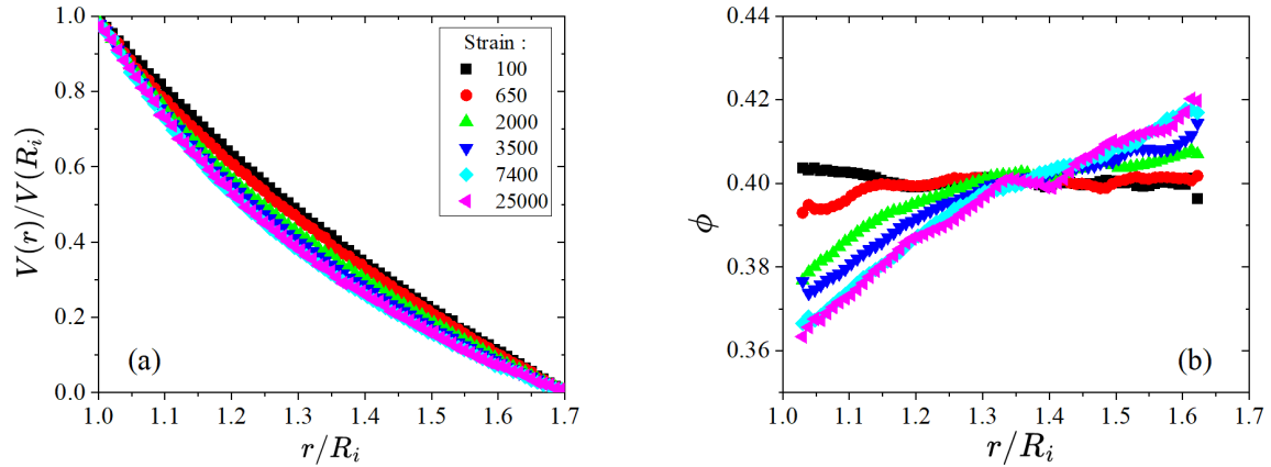
FIG. 11. Evolution of the velocity (a) and concentration (b) profiles as a function of the macroscopic strain \Gamma = \Omega t (see legend) for a 40% suspension. The concentration profiles are computed here from the velocity profiles, as described in the text.
