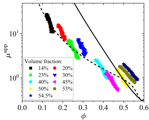
FIG. 5. Apparent friction coefficient \mu^{\text{app}} as a function of the local volume fraction \phi from experiments performed at various average volume fraction (see legend). We recall that \mu^{\text{app}} is deduced here from both the steady-state and the dynamics of migration under the assumption that there is no additional diffusion term in the SBM. The difference with Fig. 2 is that \mu^{\text{app}} is built from the steady-state volume fraction profiles only in Fig. 2c, together with a continuity hypothesis. The dashed line is the rheological laws Eq. (B3) of Boyer, Guazzelli, and Pouliquen 32 . The full line is the phenomenological laws Eq. (14).
