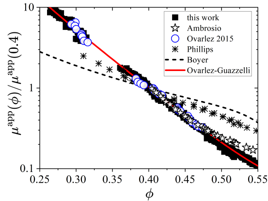
FIG. 15. Apparent friction coefficient \mu^{\text{app}} as a function of the local volume fraction \phi : comparison between our data (squares) and the data derived from the steady state volume fraction profiles of d'Ambrosio, Blanc, and Lemaire 35 (open stars), Ovarlez et al. 48 (open circles), and Phillips et al. 54 (crosses). We recall that \mu^{\text{app}} is derived under the assumption that there is no additional diffusion term in the SBM. For all experiments, \mu^{\text{app}} is rescaled by its value for \phi = 0.4 . The dashed line is the rheological law of Boyer, Guazzelli, and Pouliquen 32 , Eq. (B3). The full line is the phenomenological law Eq. (14).
