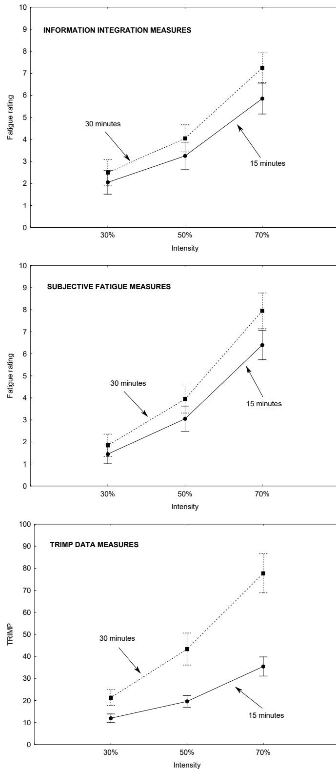
Figure 1. Effect of duration and intensity on the fatigue rating in a laboratory condition (top panel) and in a real sports condition (middle panel) and on the TRIMP in a real sports condition (bottom panel).
