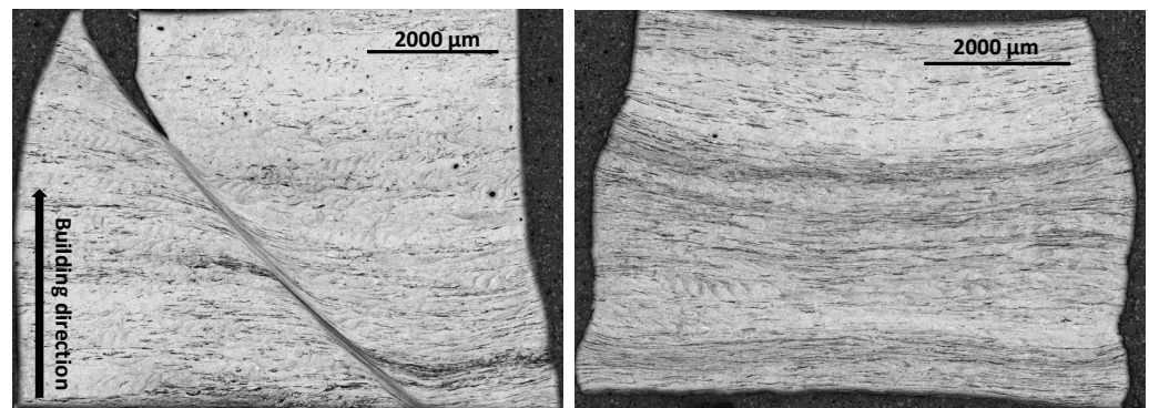
Figure 13. OM observations of Ti42Nb specimens manufactured with a building direction of 90^\circ deformed at a strain rate of 10 \text{ s}^{-1} and two temperatures: (left) 298 K and (right) 1073 K.
