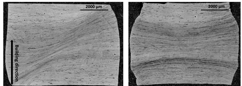
Figure 14. OM observations of Ti42Nb specimens manufactured with a building direction of 45^\circ deformed at a strain rate of 10 \text{ s}^{-1} and two temperatures: (left) 298 K and (right) 1073 K.
