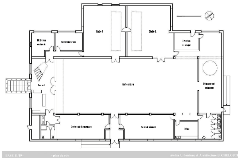
BASE 11/19 - plan de rez Atelier Urbanisme & Architecture B. CHELOUT
