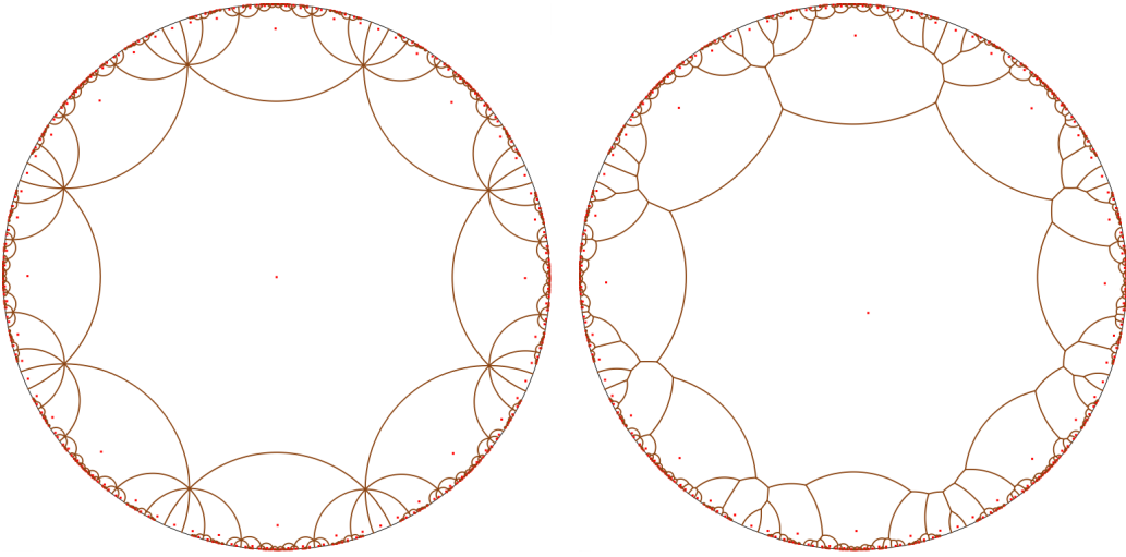
Figure 1 Dirichlet domains for the Bolza surface ( g = 2 ). The domain on the left has 4g = 8 sides and the one on the right has 12g - 6 = 18 sides. Figure from [3].
