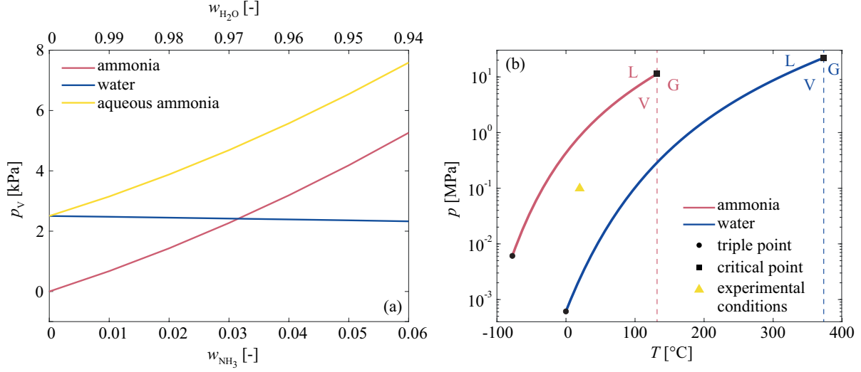
FIG. 2. (a) Total vapour pressure of aqueous ammonia solutions as a function of the mass fraction of ammonia w_{\text{NH}_3} (and relative water mass fraction w_{\text{H}_2\text{O}} ) at 21 °C from Green and Perry 32 . The plot also displays the partial vapour pressure of the solution's components. (b) Phase diagram of pure water and pure ammonia from Green and Perry 32 . The solid lines show the liquid-vapour phase boundary for both substances. The black circles indicate the triple point, whereas the black squares indicate the critical point. L, V, and G stands for liquid, vapour, and gas, respectively. The triangle indicates the experimental conditions.
