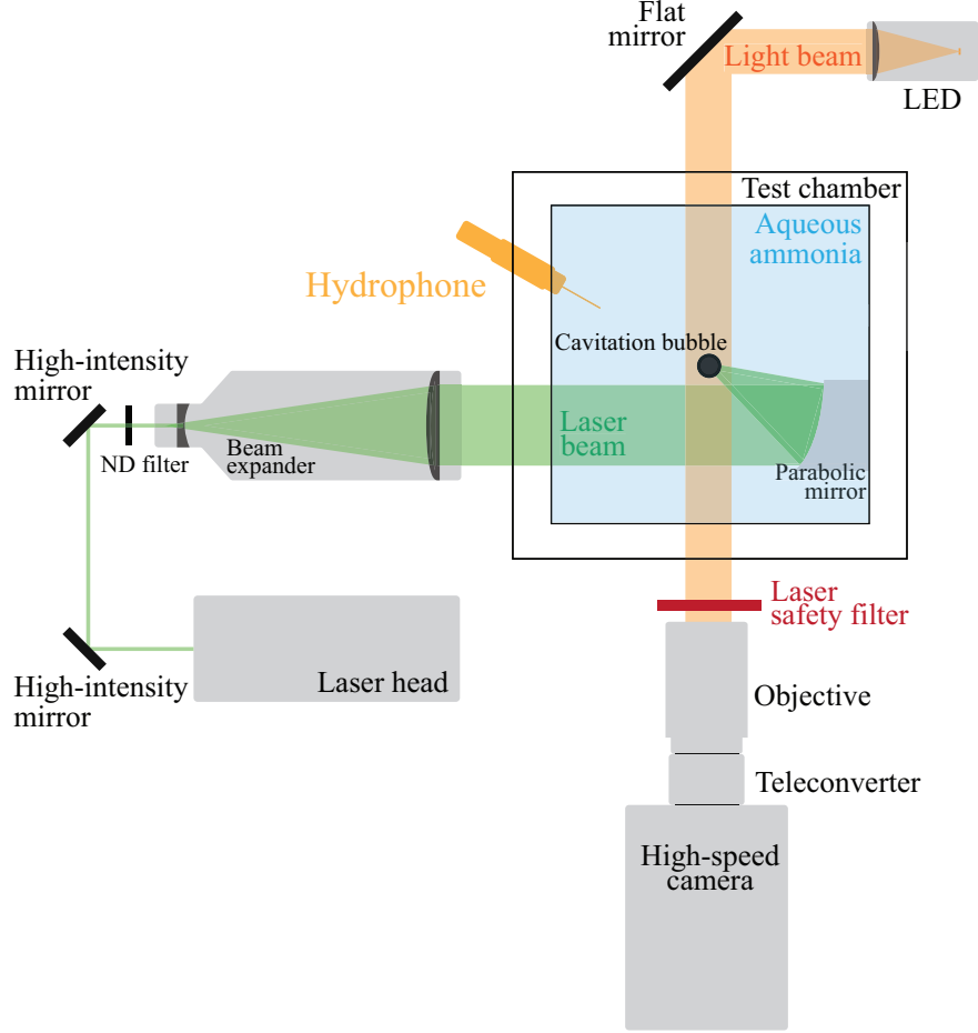
FIG. 1. Top-view schematic of the experimental apparatus.
