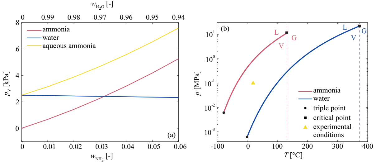
FIG. 2. (a) Total vapour pressure of aqueous ammonia solutions as a function of the mass fraction of ammonia w_{NH_3} (and relative water mass fraction w_{H_2O} ) at 21 °C from Green and Perry 32 . The plot also displays the partial vapour pressure of the solution’s components. (b) Phase diagram of pure water and pure ammonia from Green and Perry 32 . The solid lines show the liquid-vapour phase boundary for both substances. The black circles indicate the triple point, whereas the black squares indicate the critical point. L, V, and G stands for liquid, vapour, and gas, respectively. The triangle indicates the experimental conditions.
