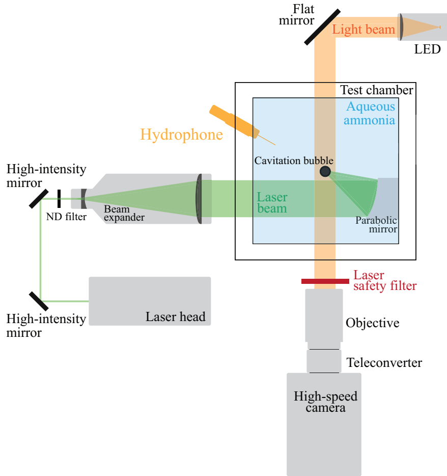
FIG. 1. Top-view schematic of the experimental apparatus.
