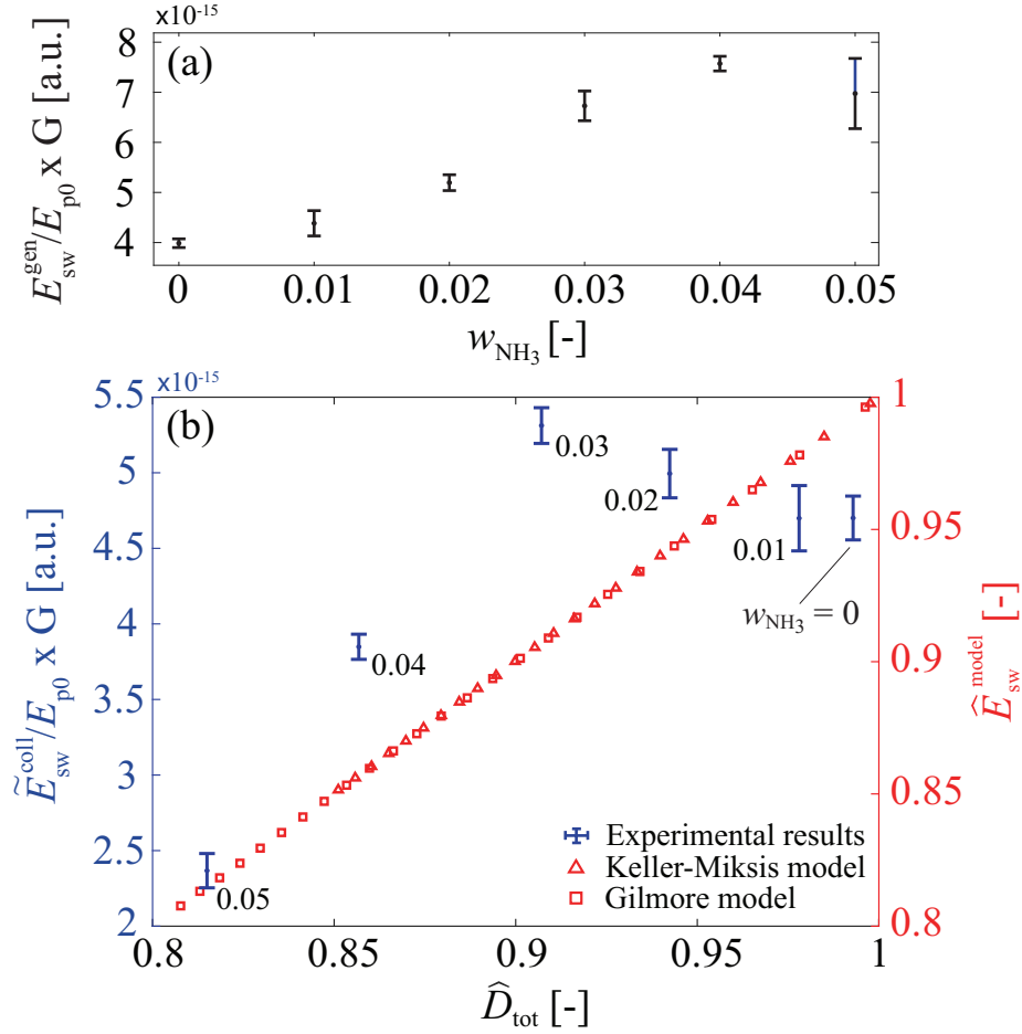
FIG. 5. (a) Energy of shock waves emitted at bubble generation, normalized by the potential energy of the bubble at maximum expansion, as a function of w_{NH_3} . (b) Energy of shock waves emitted at bubble collapse, normalized by the potential energy of the bubble at maximum expansion (experiments left y-axis, and simulations right y-axis), as a function of \hat{D}_{tot} . In both (a) and (b), points with error bars indicate the average normalized energy of the shock waves at bubble collapse obtained from 10 experiments in different aqueous ammonia with their relative standard deviation. Triangles and squares in (b) refer to the energy of shock wave at bubble collapse normalized by the potential energy of the bubble at maximum expansion obtained from simulations with the Keller and Miksis 19 model and the Gilmore 10 model, respectively, for bubbles at different initial non-condensable gas pressure p_{g0} .
