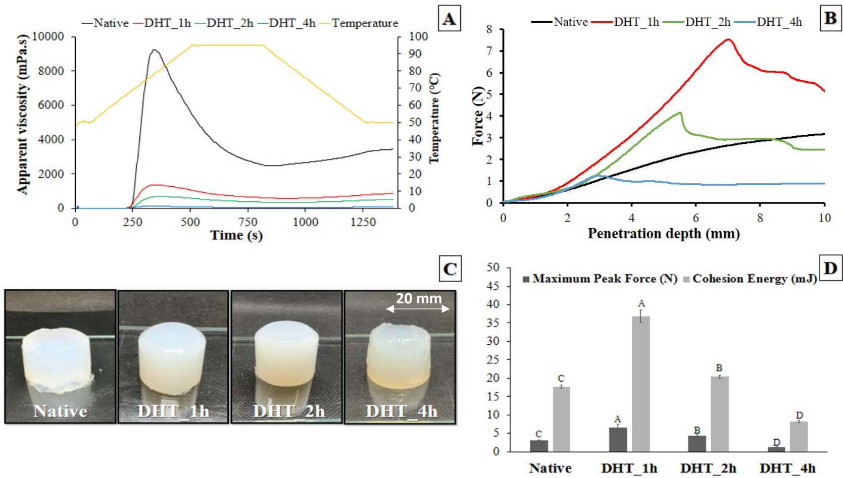
Figure 2. (A) RVA curves, (B) Force vs penetration depth, (C) images of the molded gels obtained, and (D) Maximum peak force and cohesion energy of the native and modified starches (DHT_1h, DHT_2h, and DHT_4h). A, B, C, D: different letters indicate significant differences between the native and the modified starches, as revealed by Tukey's test, p < 0.05 .
