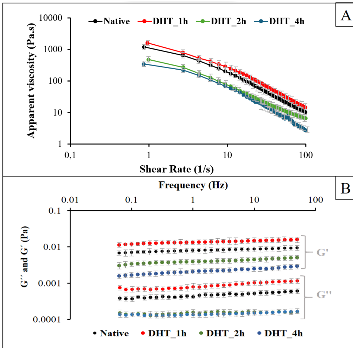
Figure 3. Rheological properties of native and DHT-modified potato starch: A) Apparent viscosity variation with the shear rate; B) Storage modulus ( G' ) and Loss modulus ( G'' ) as a function of frequency.
