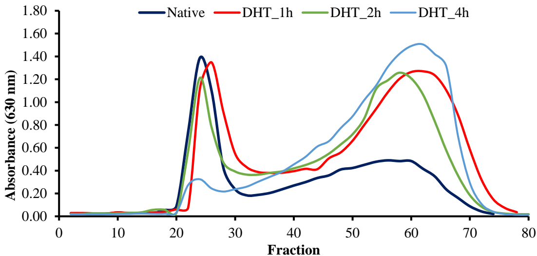
Figure 1. Molecular size distribution of the native and modified potato starches (DHT_1h, DHT_2h, and DHT_4h).
