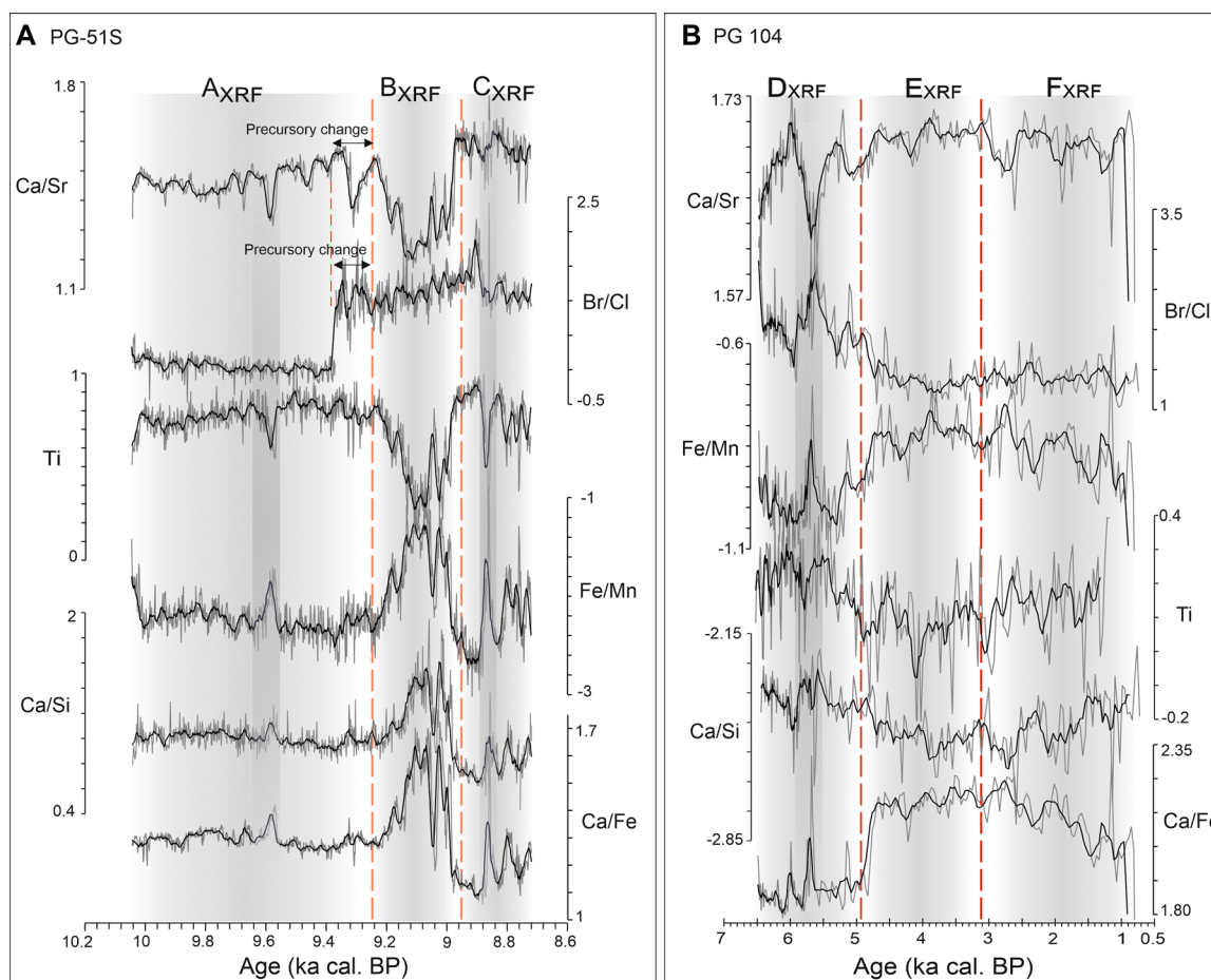
Figure 5. Variations in elemental ratios for cores PG-51S (A) and PG-104 (B). Each core shows three distinct zones of temporal changes in elemental ratios, labeled A_{XRF} , B_{XRF} and C_{XRF} for PG-51S, and D_{XRF} , E_{XRF} and F_{XRF} for PG-104. The zones are indicated by shaded areas, with darker shades representing minor, but notable, changes at 9.6, 8.9 and 5.8 ka cal BP. In A, Br/Cl and Ca/Sr ratios show notable changes before other variables that are indicated as precursory changes. The boundaries of the zones are marked by red dashed lines. [Color figure can be viewed at wileyonlinelibrary.com ]
