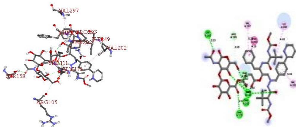
Figure 2 (e) Two dimensional interaction plot for HA-Atazanavir against ACE-2 (PDB ID 1R42)
