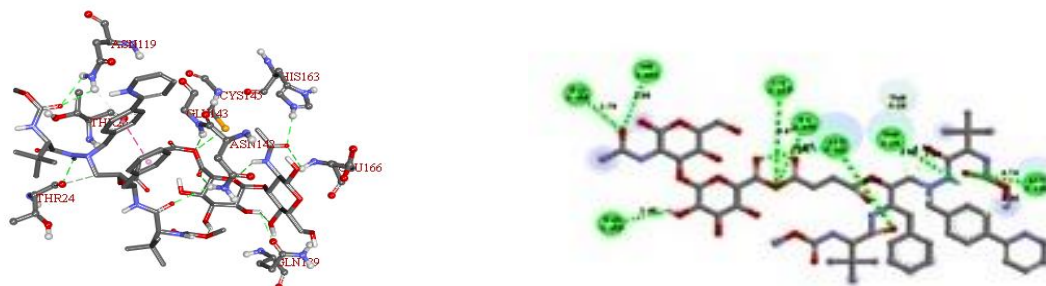
Figure 2 (b) Two dimensional interaction plot for HA-Atazanavir against Mpro (PDB ID 6M03)
