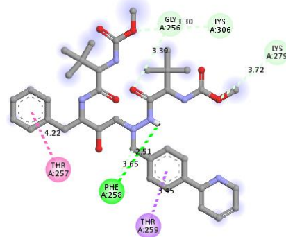
Figure 2 (c) Two dimensional interaction plot for Atazanavir against PLpro (PDB ID 6W9C)
