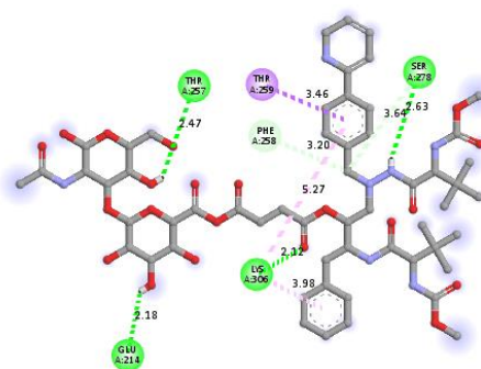
Figure 2 (d) Two dimensional interaction plot for HA-Atazanavir against PLpro (PDB ID 6W9C)
