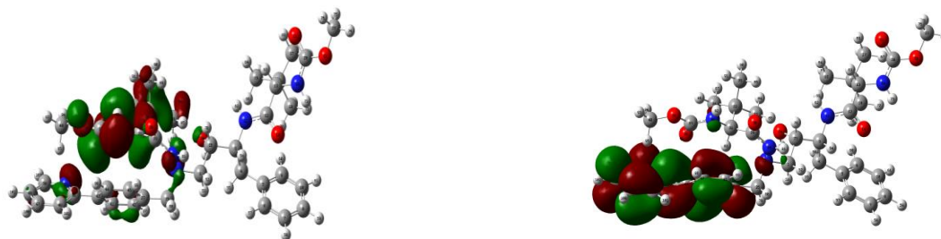
Figure 3 (a) Atazanavir HOMO orbital (b) Atazanavir LUMO orbital
