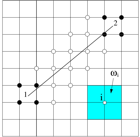
Fig. 2 Enriched nodes for an embedded crack. The crack-tips are labeled as 1 and 2. The nodes that are enriched with the discontinuous function are shown by open-circles , whereas those that are enriched with the asymptotic near-tip crack functions are shown by filled-circles . The shaded region is the support \omega_i of the nodal finite element basis function for node i
