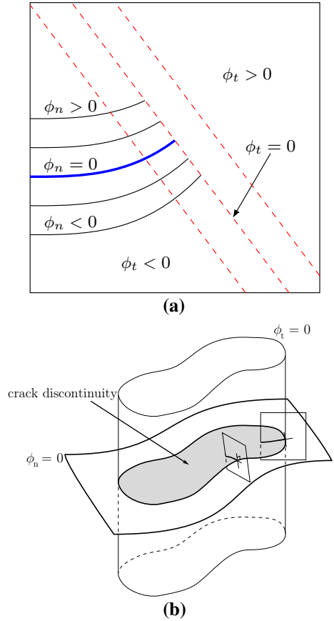
Fig. 6 Level set representation of a crack. Signed distance functions \phi_n and \phi_t to represent the crack interior and the crack tip/front, respectively. The functions are illustrated for 2D in (a) and for 3D in (b)
