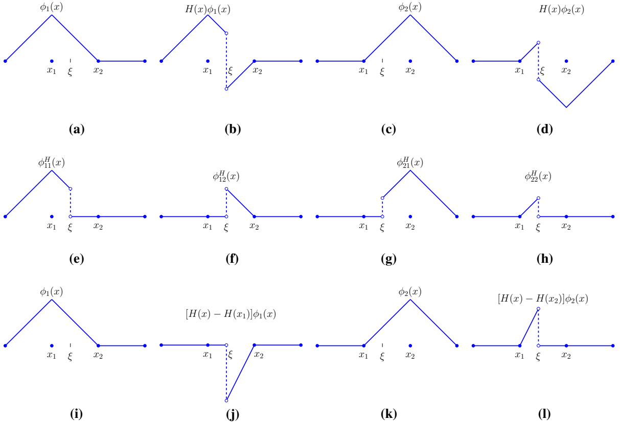
Fig. 3 Basis functions for a discontinuity in one dimension. a–d X-FEM with generalized Heaviside enrichment. e–h Approach of Hansbo and Hansbo (2004); and i–l Shifted Heaviside enrichment
