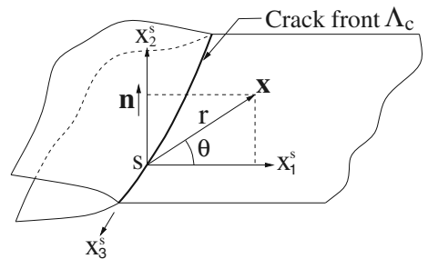
Fig. 4 Local coordinate system for crack front enrichment
