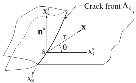
Fig. 4 Local coordinate system for crack front enrichment
