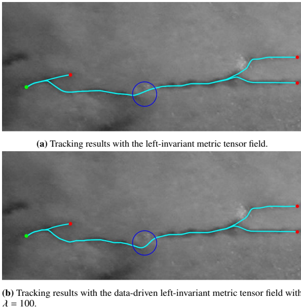
Fig. 10 Application in crack detection: Tracking results for the left-invariant and data-driven left-invariant metric tensor field on an image of cracks in a building. The presented results are calculated using 32 orientations, and parameter settings g_{11} = 0.01 , g_{22} = 1 , g_{33} = 1 . In regions with high curvature, the data-driven model adapts more gradually for curvature to get more data evidence than the left-invariant model which tends to prefer in-place rotations.
