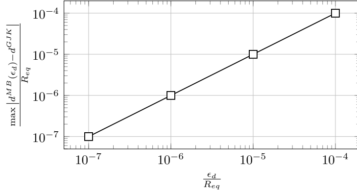
Figure F.26: Maximum error committed by the MB algorithm set with \epsilon_d , by comparison with the reference solution d^{GJK} . The maximum error is computed for all distance queries occurring in the arrays described in 4.1.1 and corresponding to l = 40 and \alpha = 0.25 (for all values of aspect ratio A_r ); it involves 2.081.738 distance queries.
