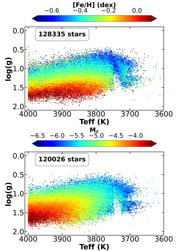
Fig. 1. Kiel diagram of the best-parameterised GSP-Spec AGB stars colour-coded by their metallicity (top panel) and their absolute K magnitude (neglecting the extinction; bottom panel). This figure uses the calibrated \log(g) and [M/H] as recommended by Recio-Blanco et al. (2023).
