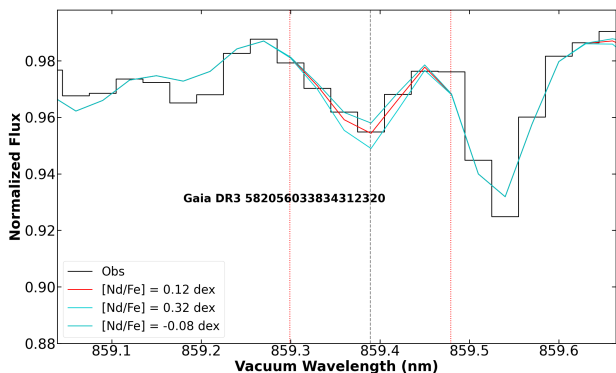
Fig. 3. Comparison around the Nd II line between the RVS public spectrum of Gaia DR3 582056033834312320 (in black) and a model spectrum computed from its GSP-Spec parameters (in red). The cyan lines show synthetic spectra with Nd abundance \pm 0.2 dex around the adopted Nd abundance. The calibrated parameters of this star are S/N = 1110 , T_{\text{eff}} = 3825 K, \log(g) = 0.37 , [\text{Fe}/\text{H}] = -0.74 dex, [\alpha/\text{Fe}] = 0.12 dex, [\text{Nd}/\text{Fe}] = 0.12 dex, and [\text{Ce}/\text{Fe}] = 0.14 dex.
