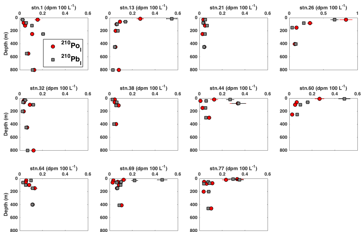
Figure 5. The vertical profiles of the particulate ^{210}\text{Po} and ^{210}\text{Pb} activity in the large size fraction ( > 53\ \mu\text{m} , ^{210}\text{Po}_I , ^{210}\text{Pb}_I ) in the top 800 m. Note that the activity scale at station 26 differs from the scale in all other plots.
