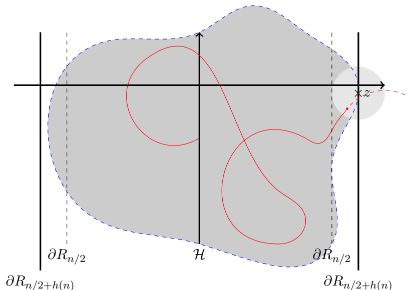
Figure 5: An example of a walk in M_{n/2+h(n)}^*(n\mathbf{1}_{\mathcal{H}_{n\gamma}}, \mathbb{B}(z, h(n)))
