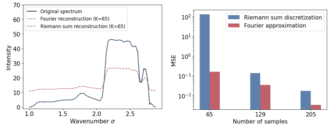
Figure 1: (left) Reconstruction of the spectrum from the measurements using the proposed approach with a Fourier basis and the implicit discretization of the integral operator on a uniform grid for 65 basis functions and 65 samples. Fourier basis functions allow for an accurate reconstruction of the spectrum even for a small number of basis functions. (right) discrete MSE (in log scale) between the ground-truth spectrum and its reconstruction from the measurements using the proposed approach with a Fourier basis and the explicit discretization of the integral operator on a uniform grid. The reconstruction precision is significantly improved using Fourier basis functions to represent the spectrum.
