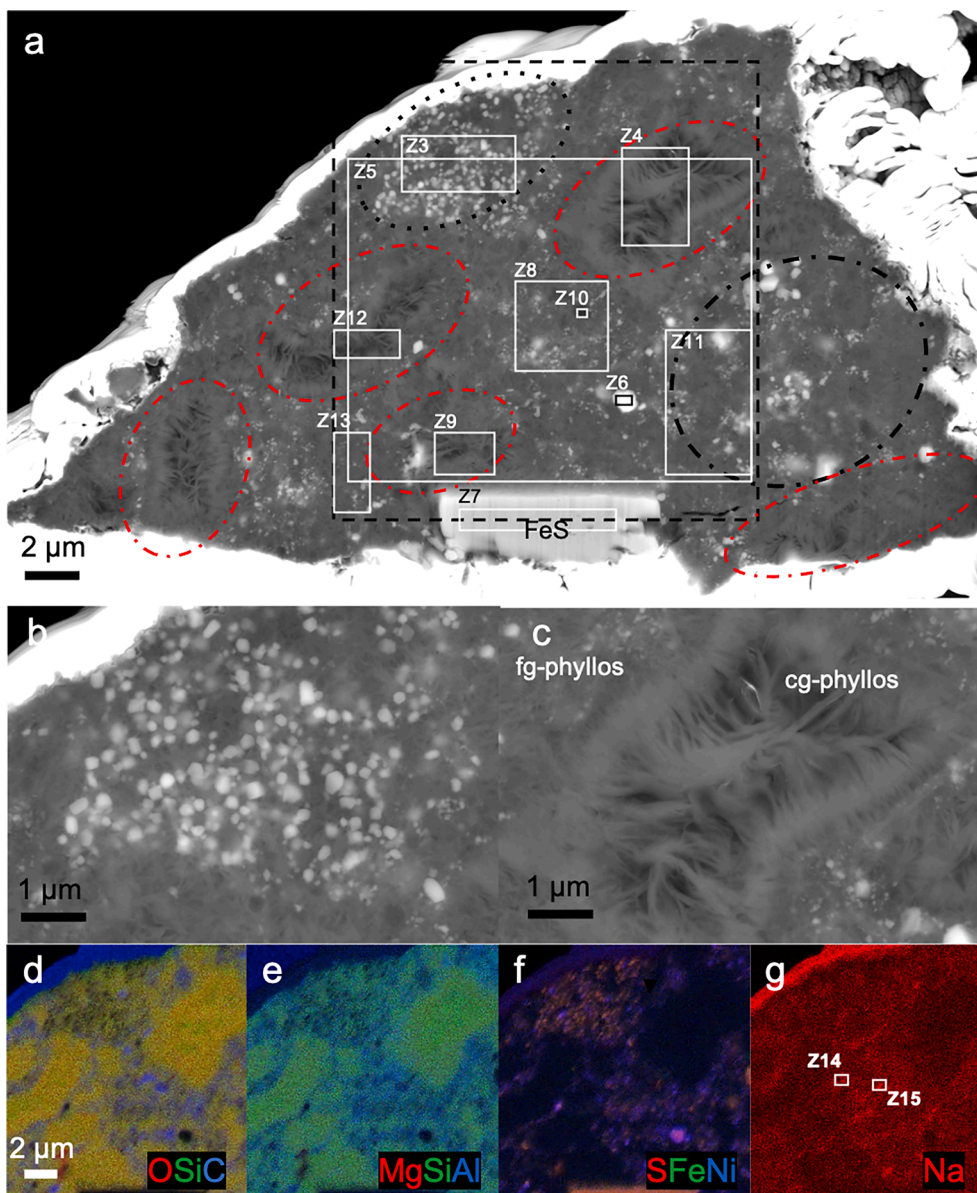
Fig. 2. a) SEM-BSE image of the thick slice extracted from grain A0064-FO019. The white layers surrounding the section correspond to the platinum deposit. b) SEM-BSE image of the fg-phyllous sulfide-rich region. Notice the euhedral morphology of the sub- \mu\text{m} sulfides. c) BSE image of the cg-phyllous. Cg-phyllous show large and oriented packets of layers radiating inward the void. d) composite X-ray map of O (red), Si (green) and C (blue) showing the very low concentration in C in the cg-phyllous. e) composite X-ray map of Mg (red), Si (green) and Al (blue). f) composite X-ray map of S (red), Fe (green) and Ni (blue) showing the presence of both Ni-rich and Ni-poor sulfide and g) X-ray map of Na distributed heterogeneously in the sample. On BSE image (a), red and black dashed-line circles indicate cg-phyllous- and fg-phyllous-rich regions, respectively. The black dashed-line rectangle indicates the analyzed zone corresponding to the X-ray maps (d-g). The numbered white rectangles correspond to zones analyzed by EDS (Table 1). Abbreviations: FeS for sulfide, cg-phyllous for coarse-grained phyllosilicates, fg-phyllous for fine-grained phyllosilicates.
