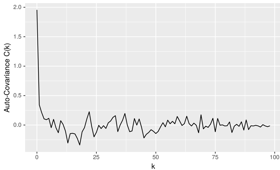
Figure 4. Auto-Covariance estimated for model (6.30) for T = 100
