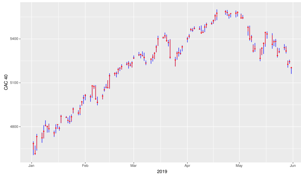
Figure 5. CAC 40 Stock Index from January 2nd to May 31st, 2019. Red arrows represent the extended intervals with left bounds the opening values (in EUR) and right bounds the closing values. The blue line segments represent the interval-valued prices composed of the lowest and highest prices of each day.
