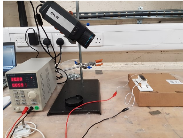
Figure 1: Experimental set-up for Joule self-heating investigation
