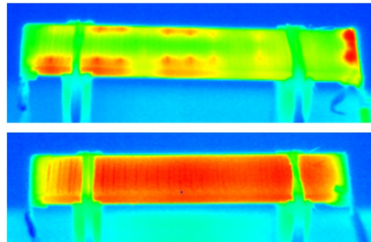
Figure 2: Temperature distribution in CP-PLA samples with high contact resistance (a) and low contact resistance (b)
