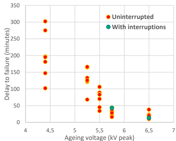
Figure 13 Delay time to failure as a function of applied voltage (30 kHz frequency). Each point is a measurement. At 4.4 kV, 5.25 kV and 5.5 kV only external discharges are present; at 5.75 kV and 6.5 kV, both internal and external discharges are present.
