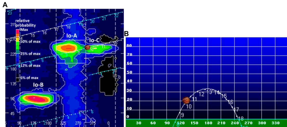
FIGURE 2 Radio Jupiter Pro features: (A) Io Phase-CML probability map with the observer’s location marked with the Jupiter planet symbol; (B) elevation of Jupiter at the location of the observer. Tick marks are labelled every hour on the tracks of Jupiter on each panel.
