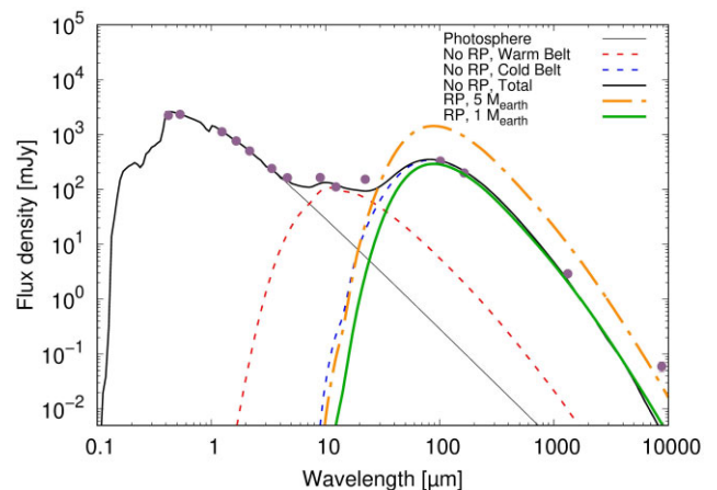
Figure 15. SED of HD 131488. The purple circles show the measured flux density at different wavelengths. The lines show models using astronomical silicate with a bulk density of 1.3 \text{ g cm}^{-3} for P = 0.6 . The blue and red dashed lines show the two component model done by the SONATA code ignoring radiation pressure. The green solid and the orange dash-dotted lines show the results from the MODERATO code where no second component was taken into account.
