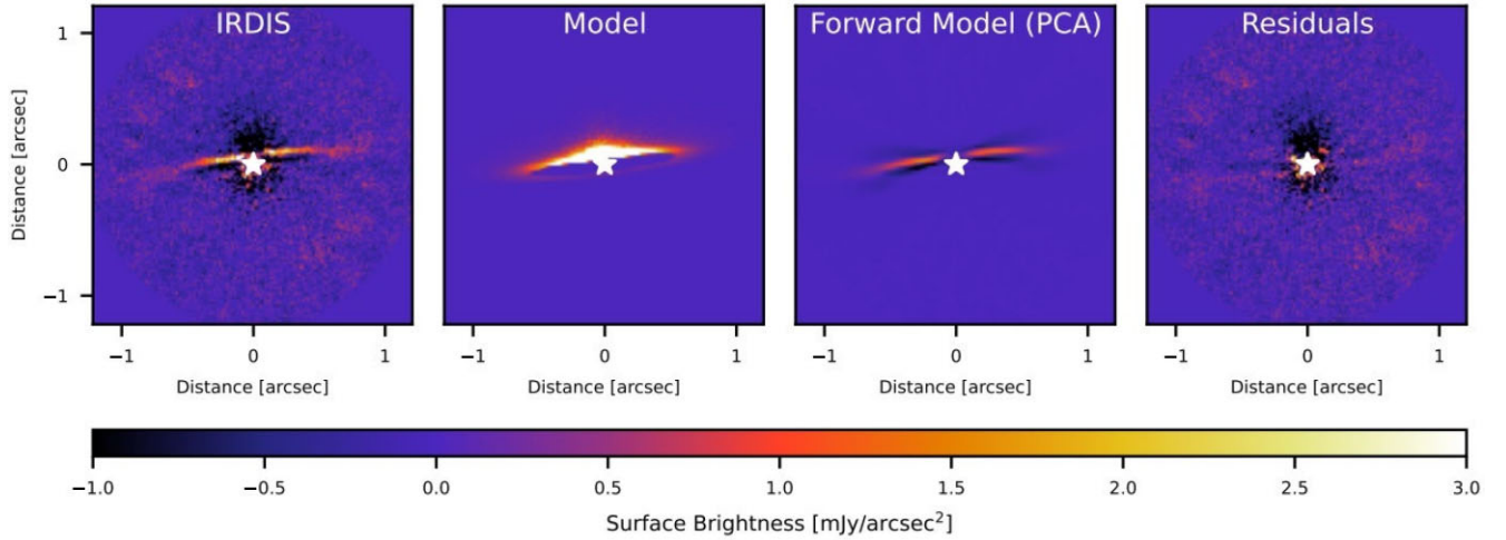
Figure 12. Best-fitting model assuming Mie theory and radiation pressure. From left to right: PCA-reduced SPHERE/IRDIS observations; model generated by MODERATO assuming P = 0.6 and q = 3.0 ; forward model (PCA); residual image.
