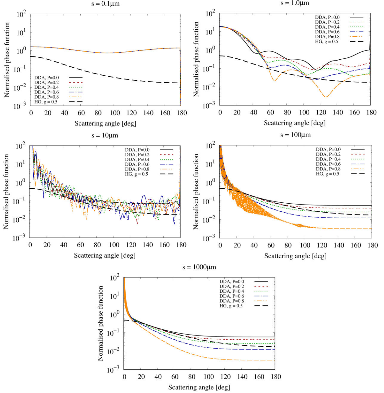
Figure A2. Scattering phase function as function of scattering angle for different porosities at a wavelength of 1.6 \mu\text{m} . The different panels show the results for different grain sizes.
