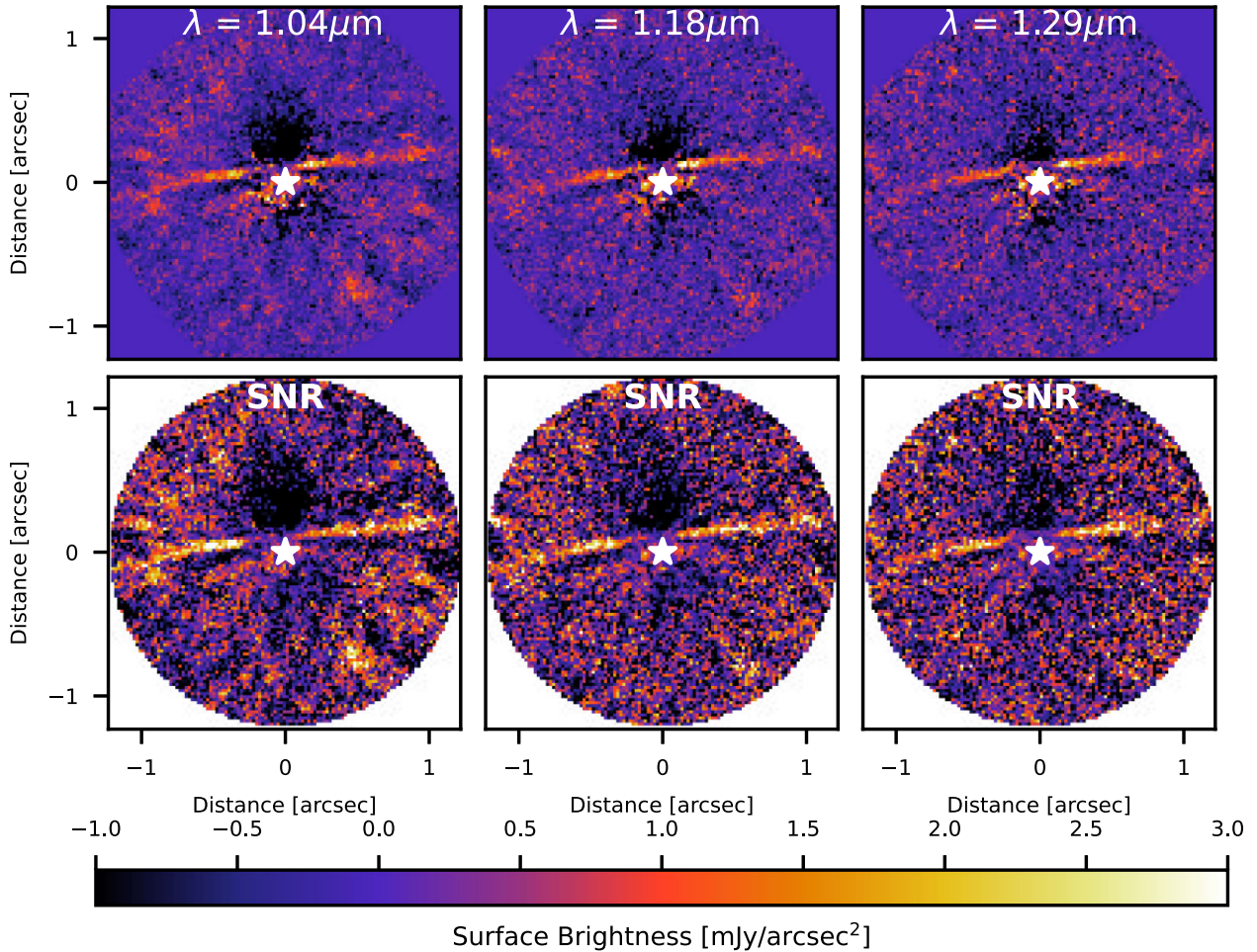
Figure 2. SPHERE/IFS data of HD 131 488 reduced with PCA and binned in the following three spectral channels (from left to right): \lambda = 1.04, 1.18, 1.29 \mu\text{m} . Top: Surface brightness maps. The surface brightness is given in \text{mJy arcsec}^{-2} . North is up and east is to the left. Bottom: SNR maps of the respective surface brightness maps.
