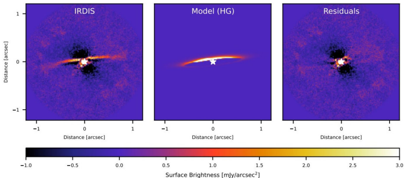
Figure 11. Best-fitting model assuming HG approximation. From left to right: PCA-reduced SPHERE/IRDIS observations; HG model; Residual image. The color scale is given in \text{mJy arcsec}^{-2} .
