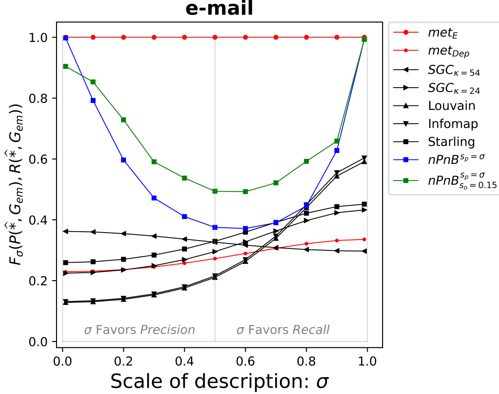
Figure 2: Performance F_{\sigma}(P(\hat{*}, G_{em}), R(\hat{*}, G_{em})) of clustering methods as derived graphs \hat{*} = \widehat{\text{met}}(G_{em}) according to the description scale \sigma .
