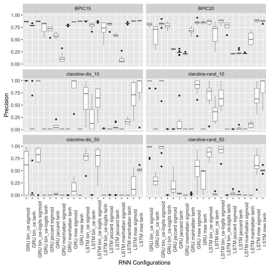
Fig. 7: Boxplots showing the Precision over 10 runs for each parametrization of each dataset.
