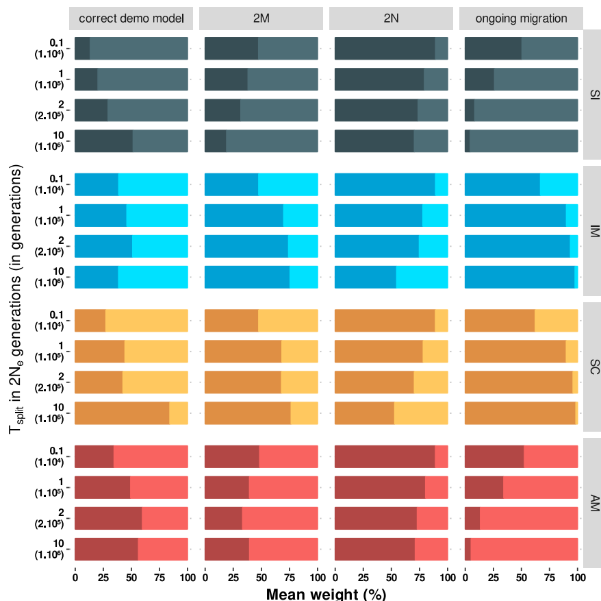
FIGURE 3 Demographic×genomic model weights in posteriors across time splits. Weight was measured by considering four criteria: (i) the average joint weight of the false and true demographic (among the four) model—called here the ‘correct’ model—in posteriors, (ii) the average joint weight of 1 m and 2 m models, (iii) the average weight of 1 N and 2 N models, (iv) and the average weight of models displaying no ongoing (current) migration and ongoing migration. Proportion of accurate model predictions are shown in dark colours. As an example, for a time split of 10^6 , an average weight of 0 for ongoing migration under the SI model signifies that across 100 replicates, simulations under ongoing migration represent 0% of the posteriors and so did not contribute to parameter estimation. All models were simulated under 2N_e m_{curr} or 4N_e m_{anc} = 1 .
