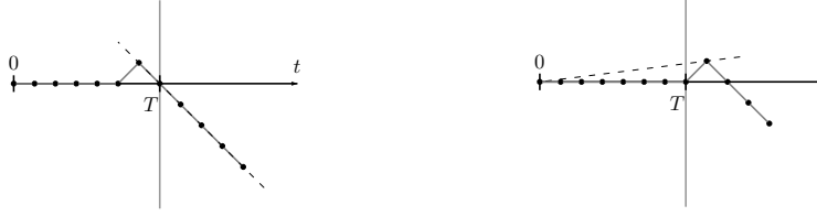
(a) Edge v_0 \rightarrow v_1 is taken too early (the sup-value is at most 0). (b) Edge v_0 \rightarrow v_1 is taken too late (the sup-value is at most \frac{T}{T+1} < 1 ).
