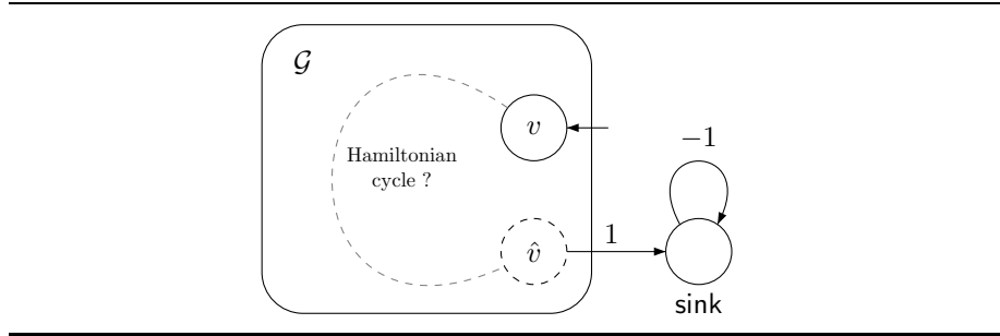
Figure 11: The NP-hardness reduction of Theorem 6.
