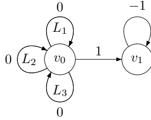
Figure 2: Three loops of respective length L_1 = 6 = 2 \cdot 3 , L_2 = 10 = 2 \cdot 5 , and L_3 = 15 = 3 \cdot 5 . For T = 32 = 6 + 10 + 15 + 1 , the optimal plan needs to visit each cycle once.
