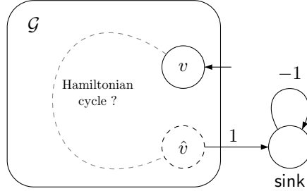
Figure 11: The NP-hardness reduction of Theorem 6.
