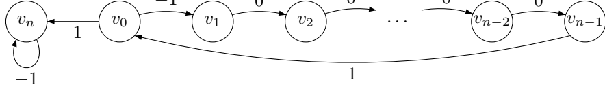
Figure 1: A weighted graph (with n+1 vertices) where the optimal path (of length T = k \cdot n + 1 ) is not simple: at v_0 , the optimal plan chooses k times the edge (v_0, v_1) , and then the edge (v_0, v_n) .
