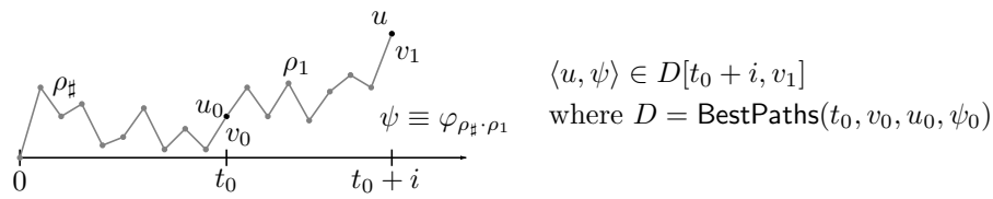
Figure 9: The result of the computation of \text{BestPaths}(t_0, v_0, u_0, \psi_0) .
