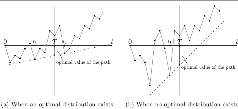
Figure 5: Geometric interpretation of the value of a path.
