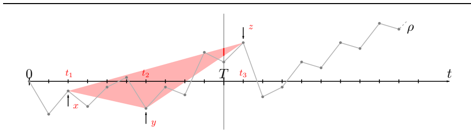
Figure 4: Bi-Dirac distributions are sufficient.
