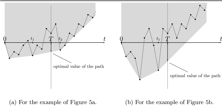
Figure 6: Convex hull interpretation of the value of a path.
