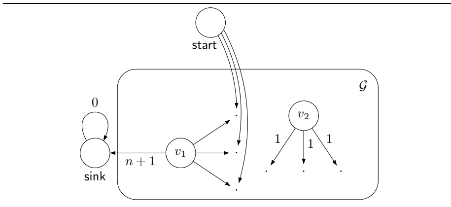
Figure 3: The NP-hardness reduction of Theorem 2.
