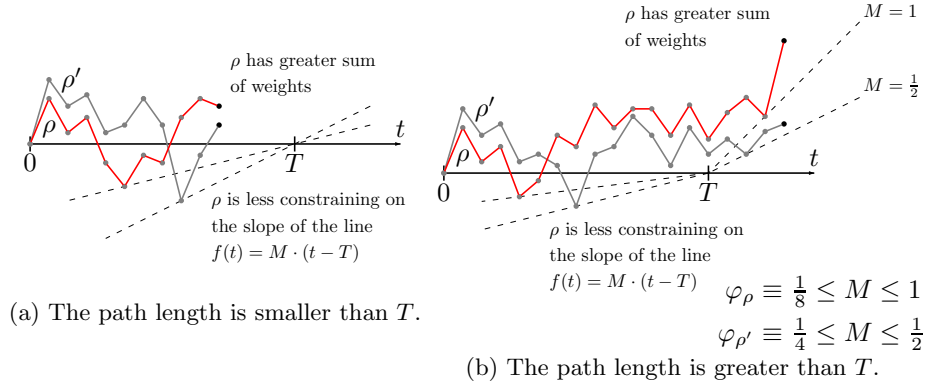
Figure 8: The path \rho is preferred to \rho' .
