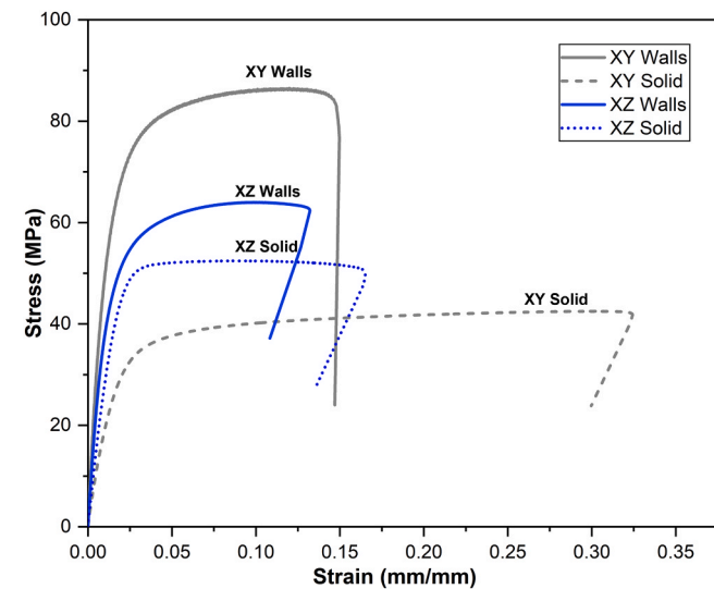
Fig. 9. Walls and solid tensile curves for XY and ZX positioning.
