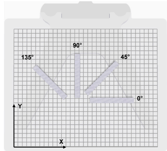
Fig. 3. Parts orientation on the printing platform.
