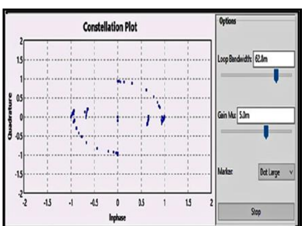
Fig. 7: Constellation plot
