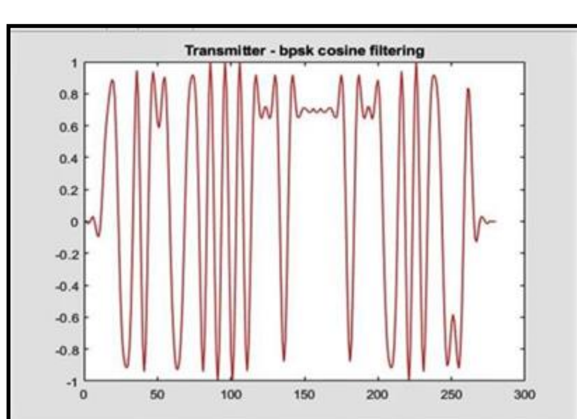
Fig. 3: BPSK cosine filtering
