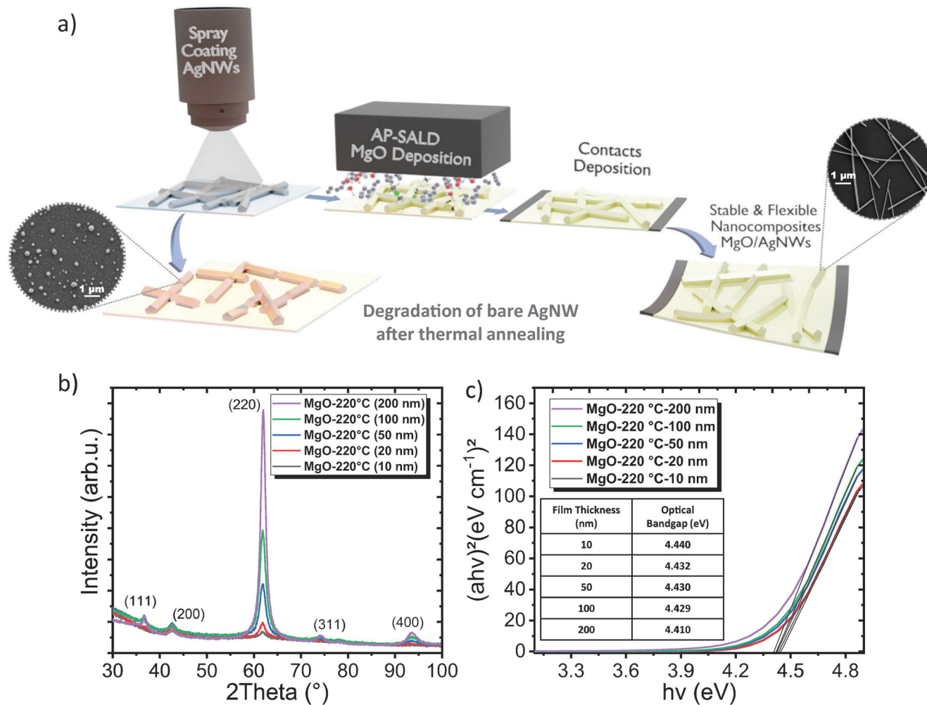
Figure 1. a) Schematic illustration presenting the fabrication steps of stable and flexible MgO/AgNW nanocomposites, by spray coating for AgNW and AP-SALD for MgO film, respectively. As shown in the SEM images in circles, bare AgNW networks degrade after thermal annealing up to 400 °C with 5 °C min -1 while the encapsulation with MgO protects them efficiently. b) XRD pattern and c) optical bandgaps, of MgO thin films with different thicknesses (from 10 to 200 nm) deposited at 220 °C by AP-SALD on glass substrate.
