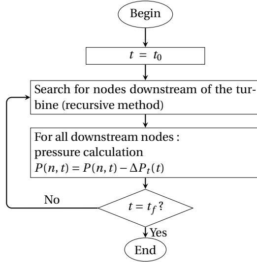
Figure 5: Algorithm for simulating the addition of a turbine.
