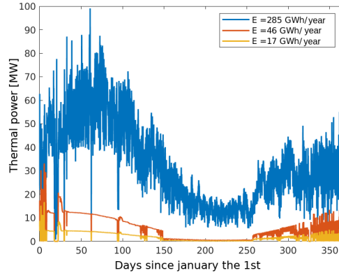
Figure 12: Thermal power that can be recovered on network A for cooling with T_{max} = 25^{\circ}\text{C} . The legend value correspond to the potentials displayed in figure 11
