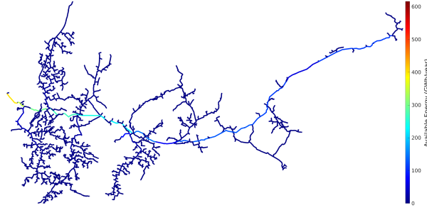
Figure 10: Network A layout colored according to the available thermal energy for heating (with T_{min} = 4^{\circ}C ).
