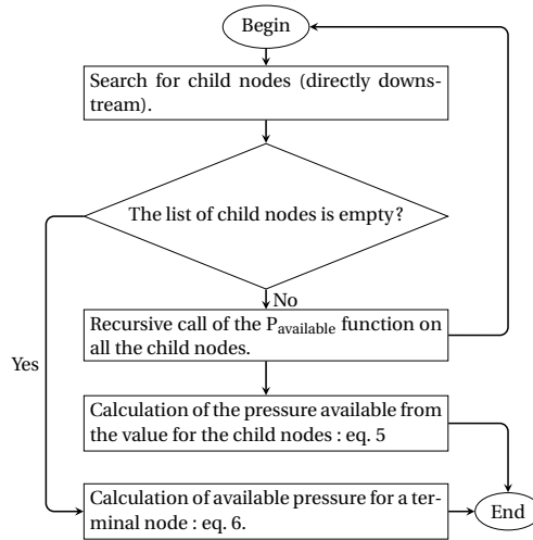
Figure 6: Algorithm for the pressure calculation
