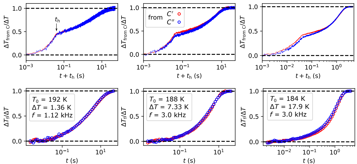
FIG. S4. Normalized temperature obtained by mapping the capacitance C'(t) (red) and C''(t) (blue) with the equilibrium values (top) and normalized fictive temperature (bottom) for three temperature steps of increasing amplitude (left to right).
