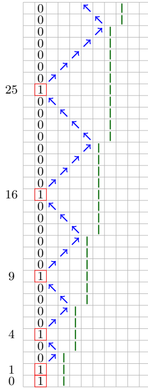
Fig. 2. Construction of (s_1(n))_{n \geq 0} by a cellular automaton
