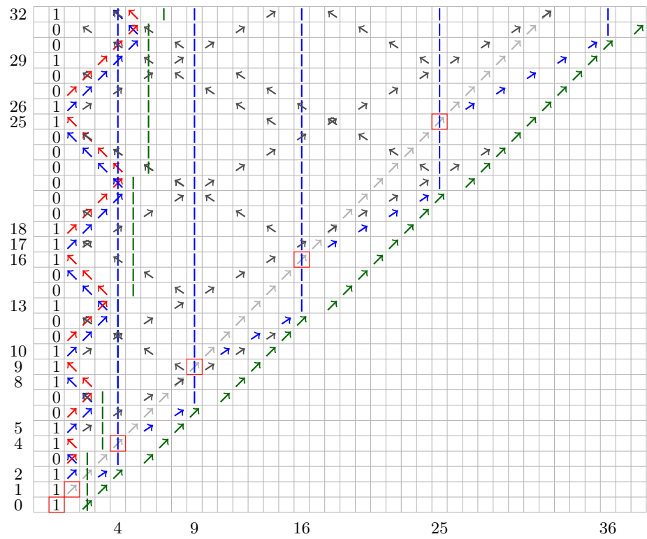
Fig. 3. Construction of (s_2(n))_{n \geq 0} by a cellular automaton
