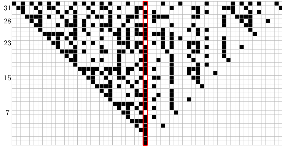
Fig. 4. Construction of (s_3(n))_{n \geq 0} by a cellular automaton
