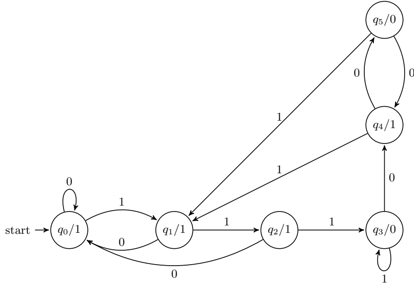
Fig. 1. A finite automaton generating the sequence (s_3(n))_{n \geq 0}
