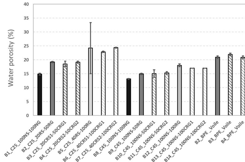
Figure 9. Water porosity.
