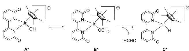
Scheme 3. Proposed generation of the anionic hydride species [\text{Cp}^*\text{Ir}(\text{bpyO}_2)\text{H}]^- ( C* ).
