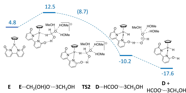
Figure 5. DFT-calculated energy profile ( \Delta G_{\text{MeOH}/298\text{K}} , \text{kcal mol}^{-1} ) and structures for the dehydrogenation of the \text{CH}_2(\text{OH})\text{O}^- \cdots 3\text{MeOH} ion promoted by the \text{Cplr}^{\text{III}}(\text{bpyO}_2) system.
