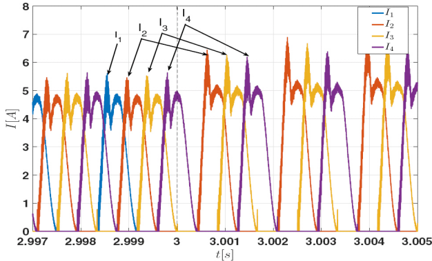
Fig. 5: Stator current responses of the SRM.
