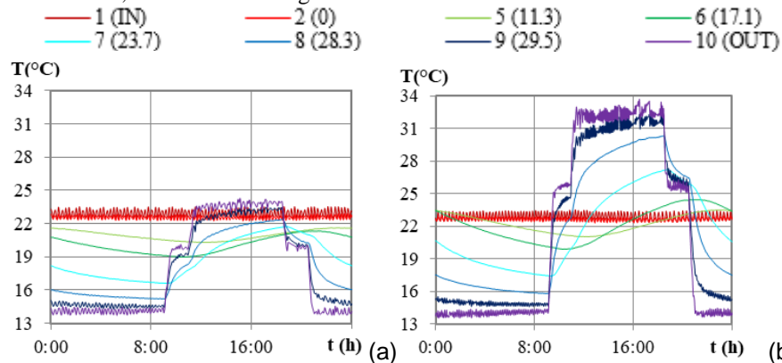
Fig. 5. Kinetics of temperature at several depth in the wall – a : without solar gains, b : with solar gains
