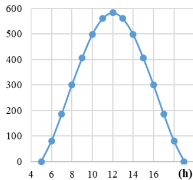
Fig. 2. Solar radiation for one typical day in Rennes in August ('Diagramme Solaire Interactif' 2022)
